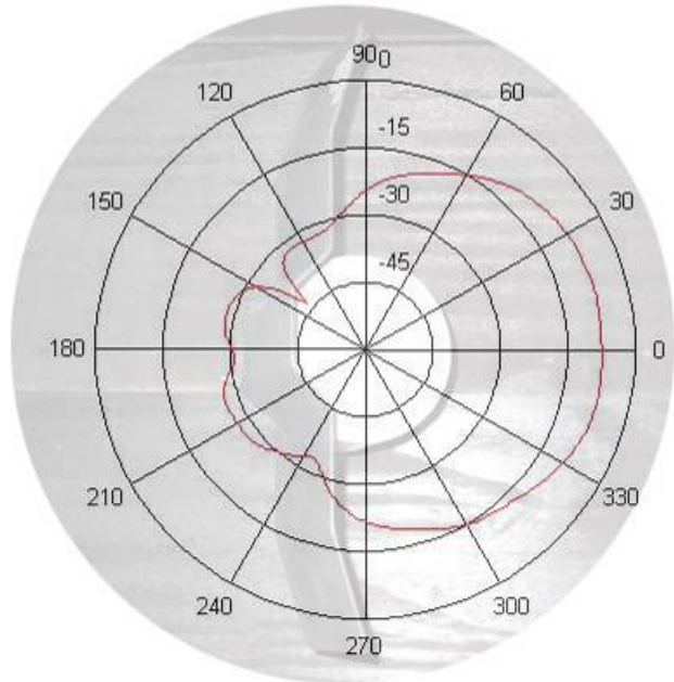
Figure 63. WiFi-Plus MP Tech 13dBi Single Sector, E-Plane at 2.4GHz
