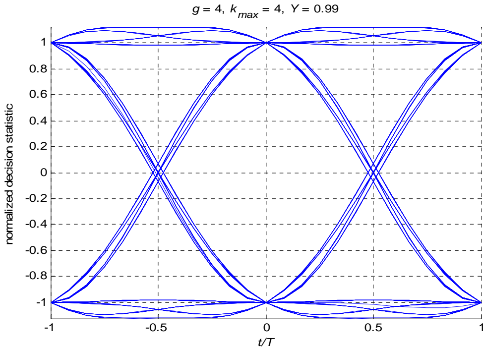
Figure 23 Eye diagram of waveform at the matched filter output for system using the new pulse with duration 4T and Y = 0.99 .
