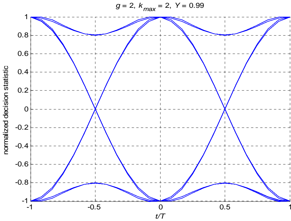
Figure 21 Eye diagram of waveform at the matched filter output for system using the new pulse with duration 2T and Y = 0.99 .
