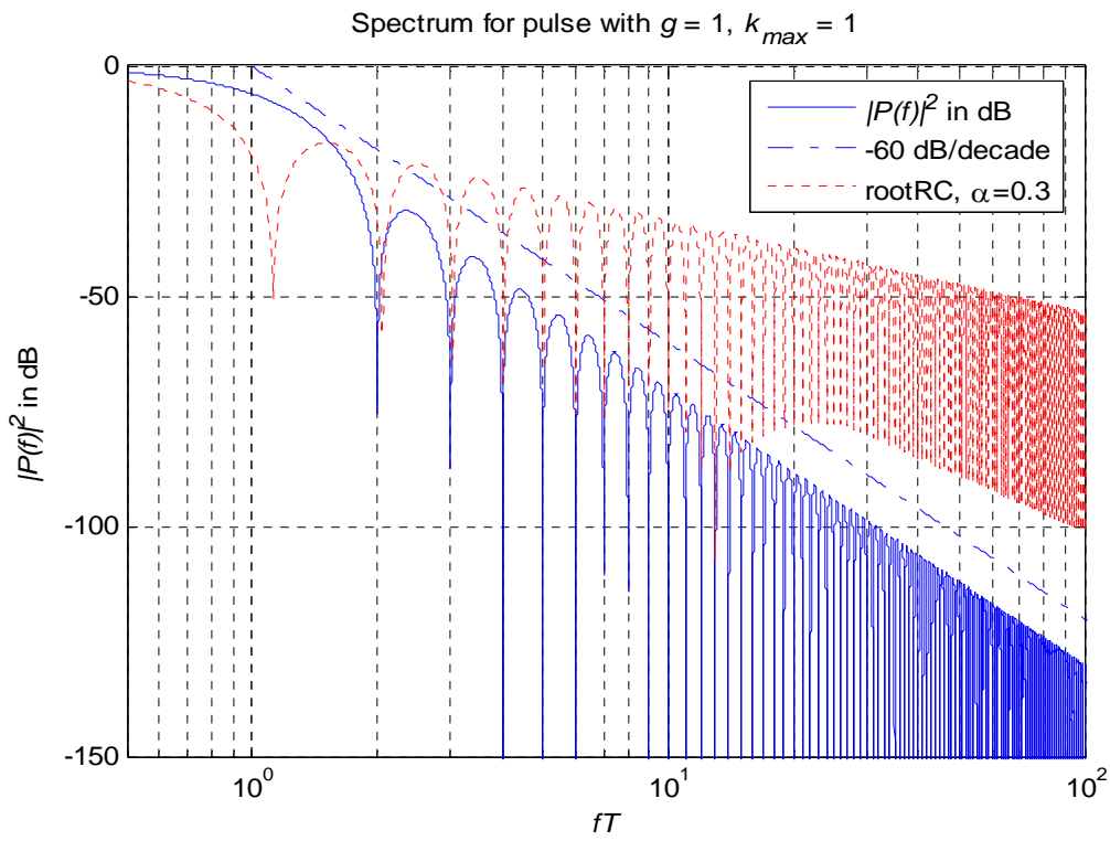
Figure 5 Comparison of duration T , new (with k_{max} = 1 ) and truncated root raised cosine (with \alpha = 0.3 ) pulse shapes.
