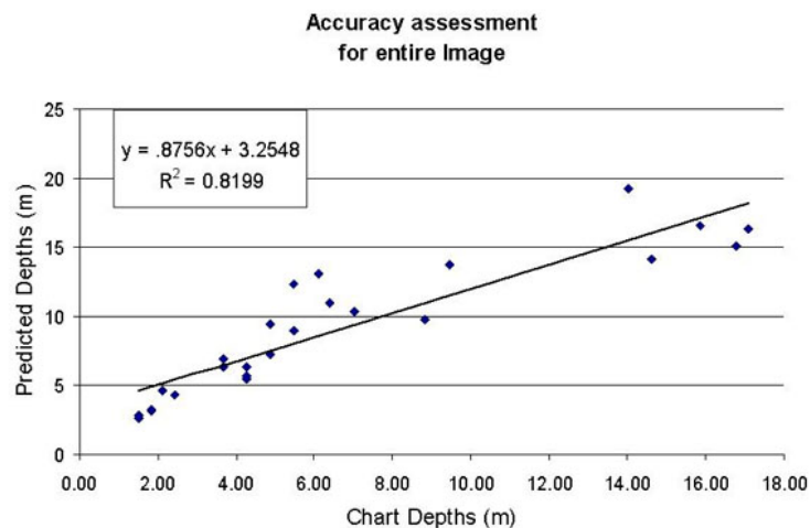
Figure 31. The absolute bathymetry when regressed against the chart depth explains 82% of the variation around the mean.
