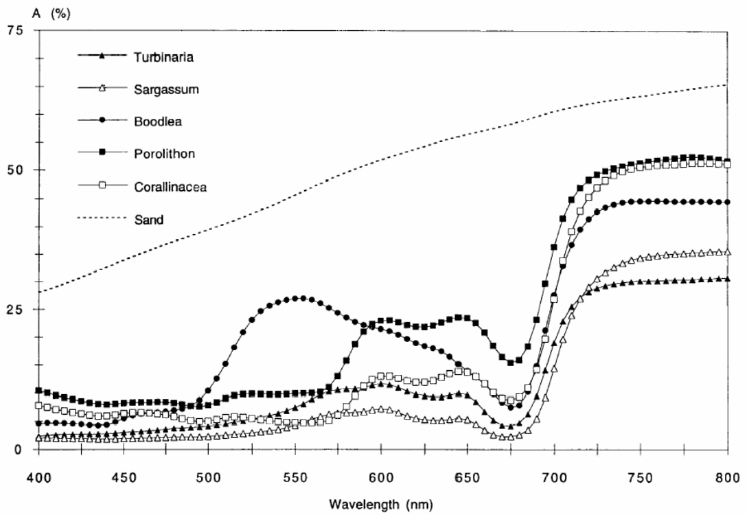
Figure 4. Albedo values for different forms of algae and coral (From Maritorena et al., 1994).
