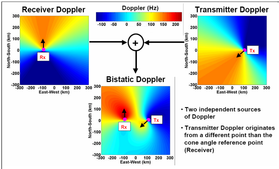
Figure 13 Isodoppler Contours from Bistatic radar (From Ref. [14])
