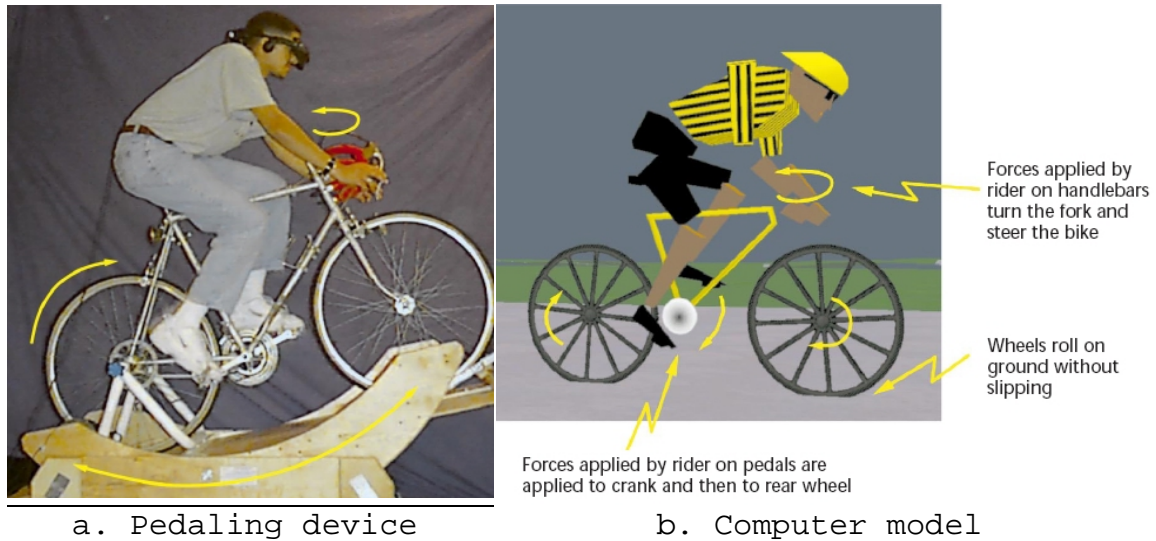
Figure 4. Pedaling device examples. Photos courtesy of Brogan, Metoyer and Hodgins, College of Computing, Georgia Institute of Technology.
