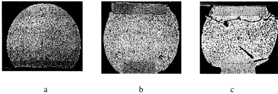
Figure 3. Flip chip joint of Sn-Ag-Cu solder after (a) 2 re-flows, (b) and (c) 2 re-flows followed by 150 thermomechanical cycles between -55\text{ }^{\circ}\text{C} and 125\text{ }^{\circ}\text{C} , with (c) being subjected to twice the shear strain range as (b), from reference [4].
