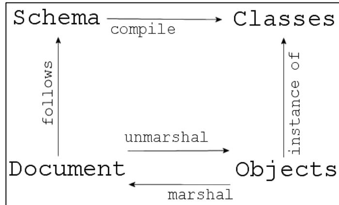
Figure III-2. XML and Java Relationships. From Ref. [Sun01].
