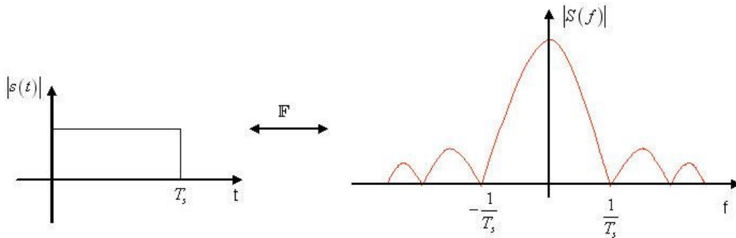
Figure 7. Representation of an OFDM Sub-Carrier: (a) In Time Domain (B) Frequency Domain
