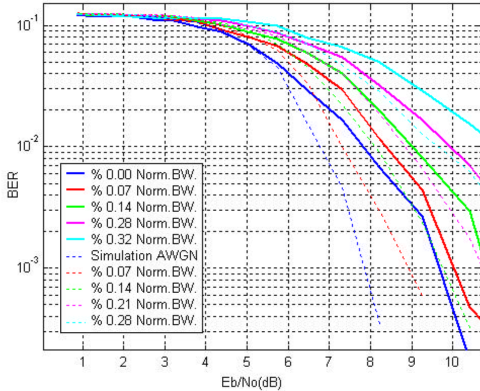
Figure 35. BER versus E_b/N_o Plots for QPSK in Mobile Channel 1 with Normalized Bandwidth \mathbf{b}/R_s Values from 0.0% to 0.28%.
