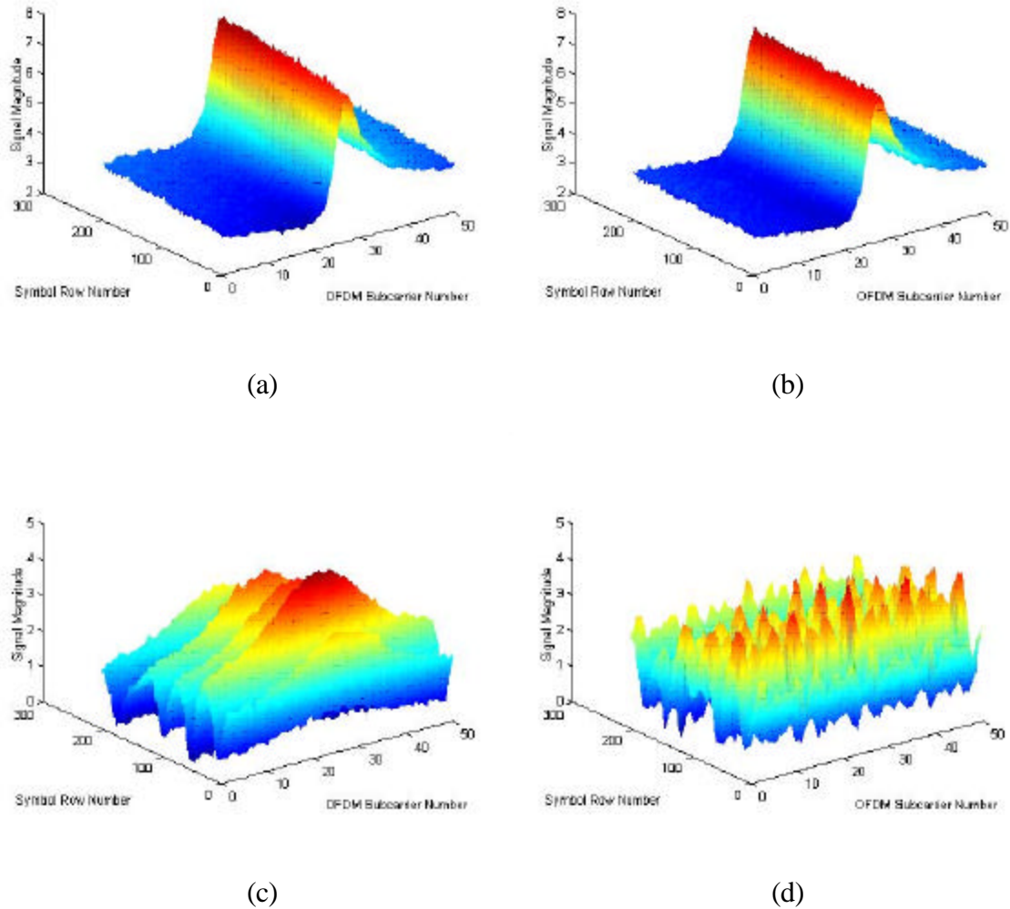
Figure 25. Effect of Mobile Channels on the Magnitude Plot of Received Symbols. (a) Mobile Channel 1 (b) Mobile Channel 2 (c) Mobile Channel 3 (d) Mobile Channel 4.
