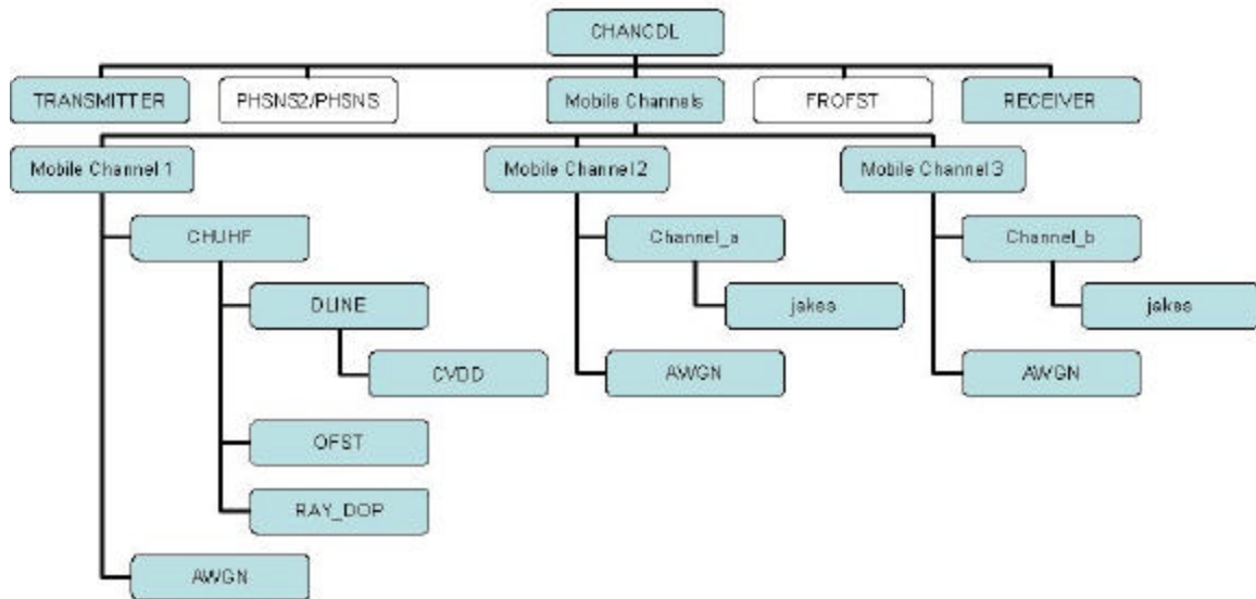
Figure 39. Mobile Channels m-file Hierarchy
