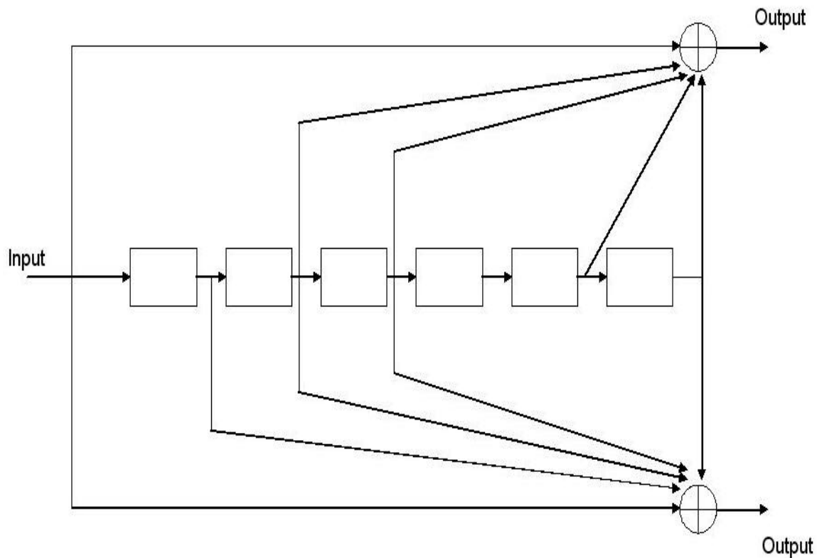
Figure 10. Convolutional Encoder with Constraint Length= 7. Each box represents a shift register (After Ref. 11.)
