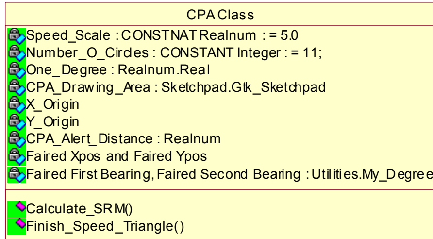
Figure 17. CPA Class
