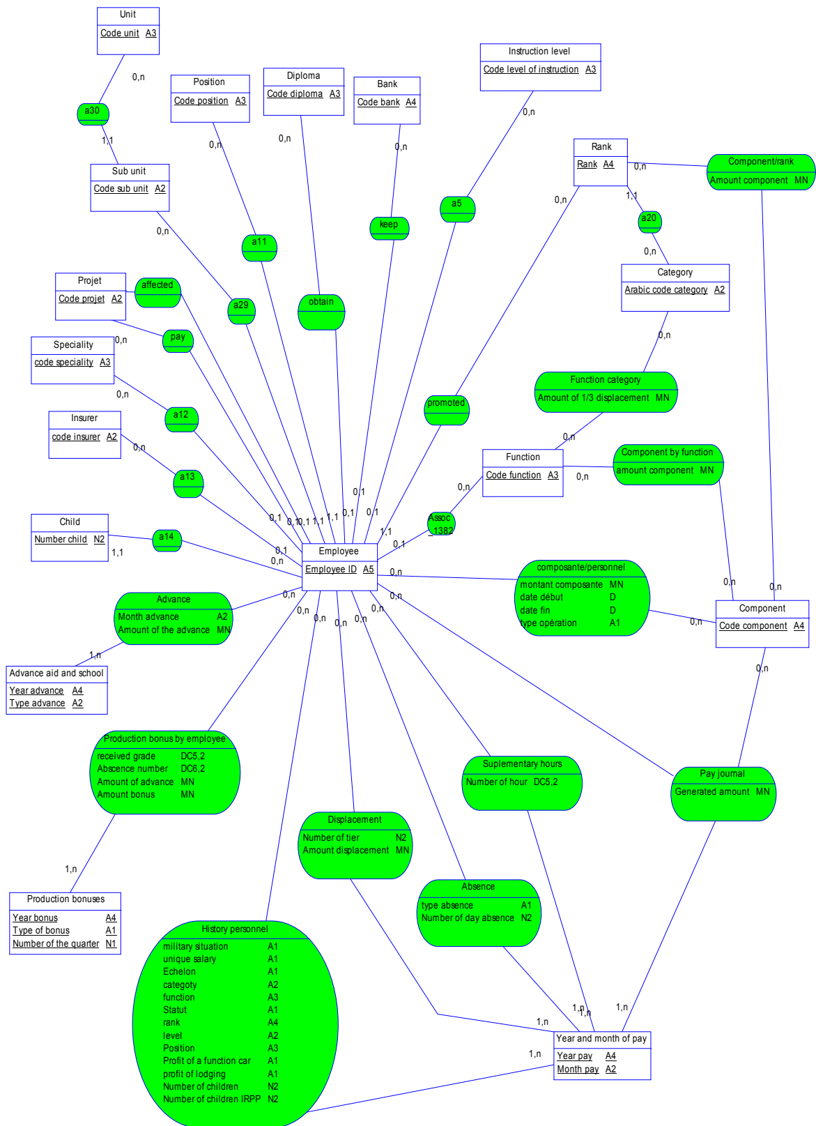
Figure 7. Conceptual Data Model Representation for Order Payoff of Personnel
