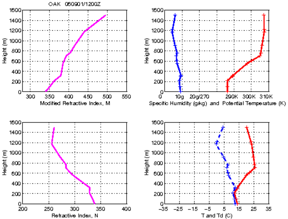
Figure 21. Example of profiles of atmospheric and refraction parameters from the 0500 PDT Oakland radiosonde. A similar plot was produced each day. This allows the easy detection of ducts and other refractive features.
