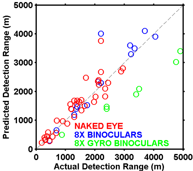
Figure 20 Comparison of predicted (NPSVIZ model) visible detection ranges with observed detection ranges for various size target features.
