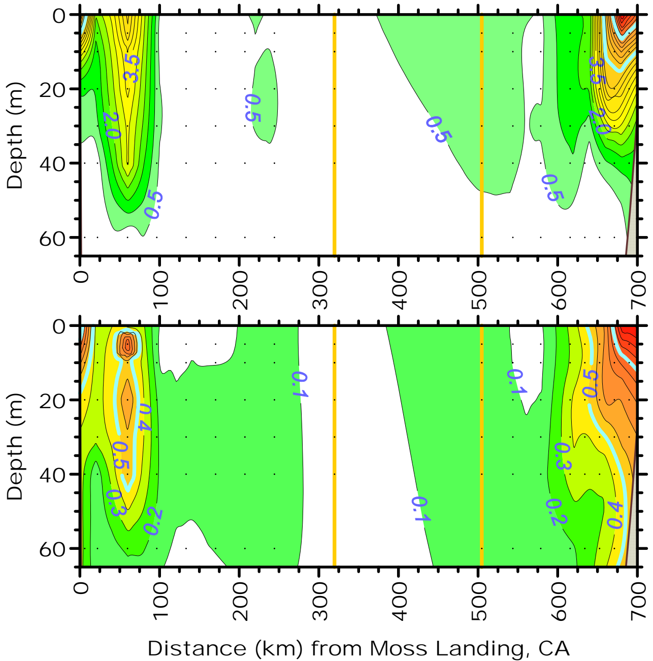
Figure 11: Contours of chlorophyll- a ( \text{mg m}^{-3} \text{ day}^{-1} ) [upper panel] and phaeophytin ( \text{mg m}^{-3} \text{ day}^{-1} ) [lower panel] in the upper 65 m of the water column along the line of hydrographic stations from Moss Landing (on the left) to Drake's Bay, California. Dots indicate the water sample locations; the yellow lines show the locations of the corner stations (CTDs 20/21 and 22). The contour intervals are 0.5 and 0.1 \text{mg m}^{-3} \text{ day}^{-1} , respectively, for the upper and lower panels. 6.0 and 9.0 (upper), while 0.5 and 1.0 (lower), \text{mg m}^{-3} \text{ day}^{-1} contours are highlighted.
