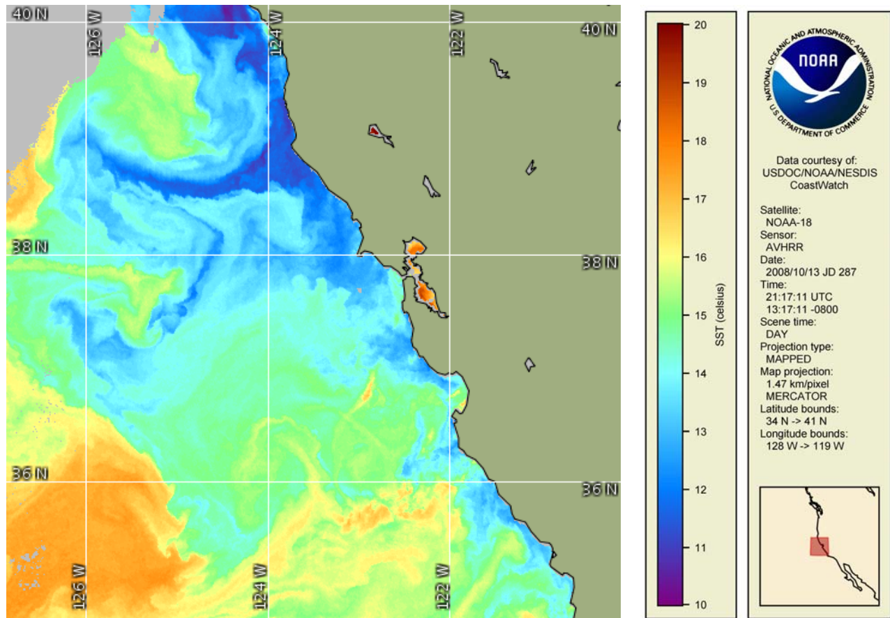
Figure 6. Advanced Very High Resolution Radiometer (AVHRR) satellite imagery of sea surface temperature ( ^{\circ} C) of the area of operation during the PaCOOS cruise of October 2008. This image was taken on 13 October 2008 at 2117 UT.
