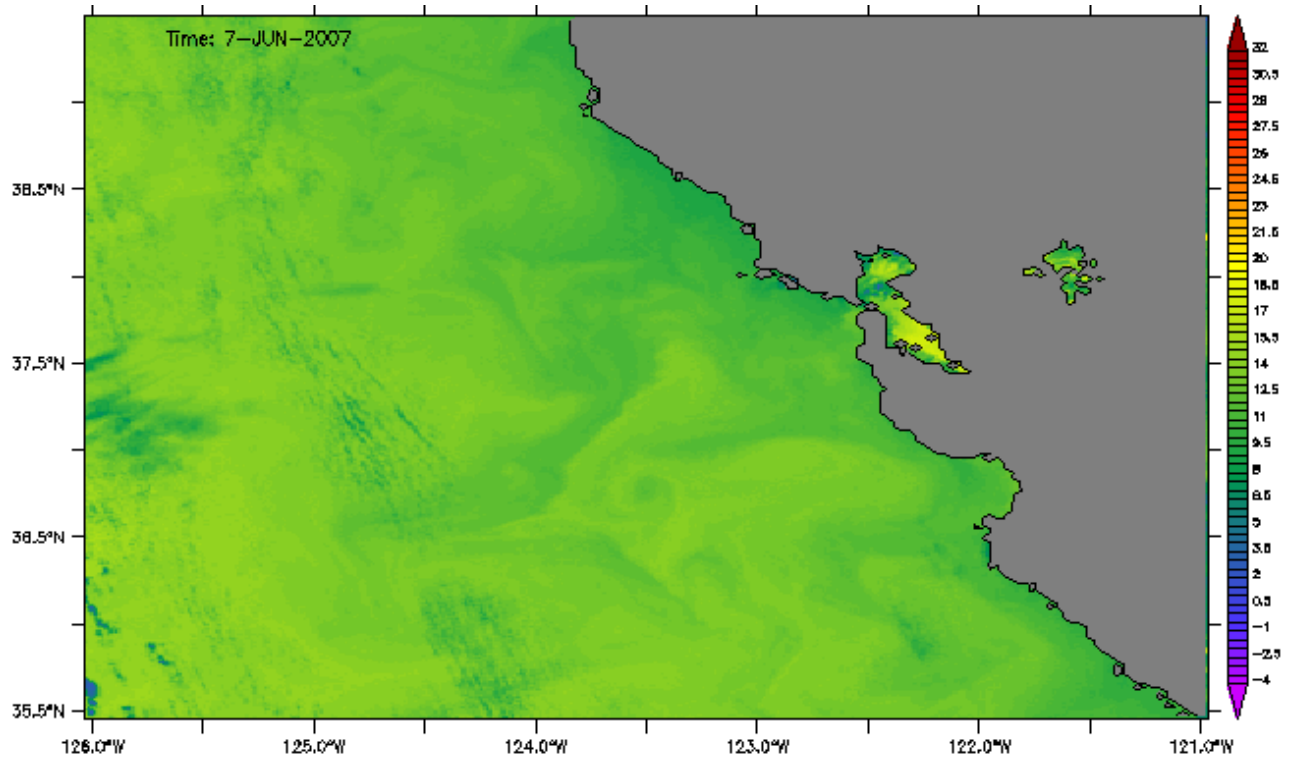
Figure 10: AVHRR (Advanced Very High Resolution Radiometer) satellite image of sea surface temperature ( ^{\circ}\text{C} ) of the area of operation during the PaCOOS cruise of June 2007. The image was taken on 7 June 2007 at 1005 UT.
