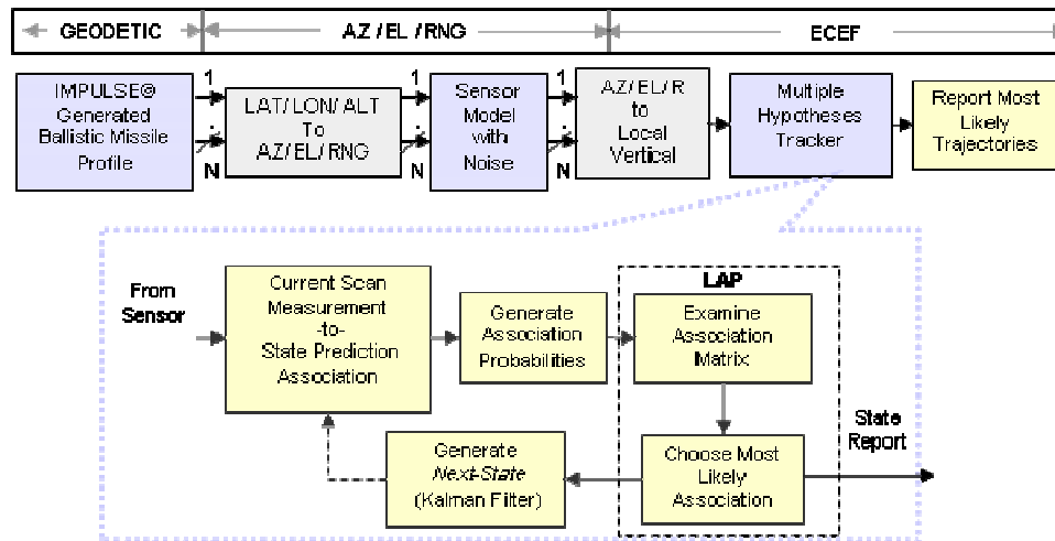
Figure 15: Main functional areas implemented in this study to include the IMPULSE© threat profile, the RF sensor model, and the multiple hypothesis tracking algorithm
