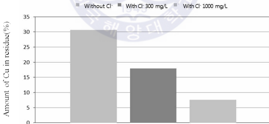
Fig. 15 Amount of Cu in residue with variation of Cl - concentration
