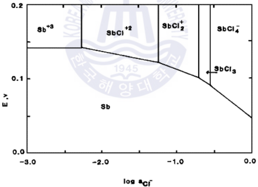
Fig. 35 Eh-log[Cl - ] diagram of the Sb-Cl-H 2 O system at 25°C and pH with activities of 10 -5 M for all soluble Sb species(Lin, 2004)
