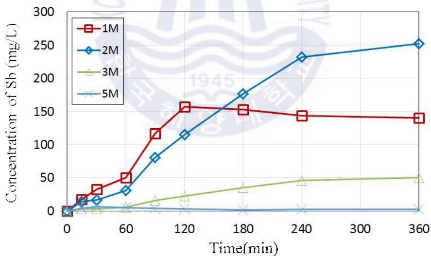
Fig. 33 Effect of HCl concentration on the concentration of Sb from Cu speiss
