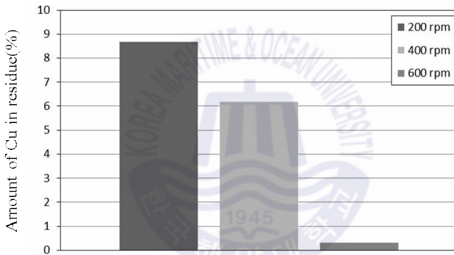
Fig. 31 Amount of Cu in residue with agitation speed and O_2
