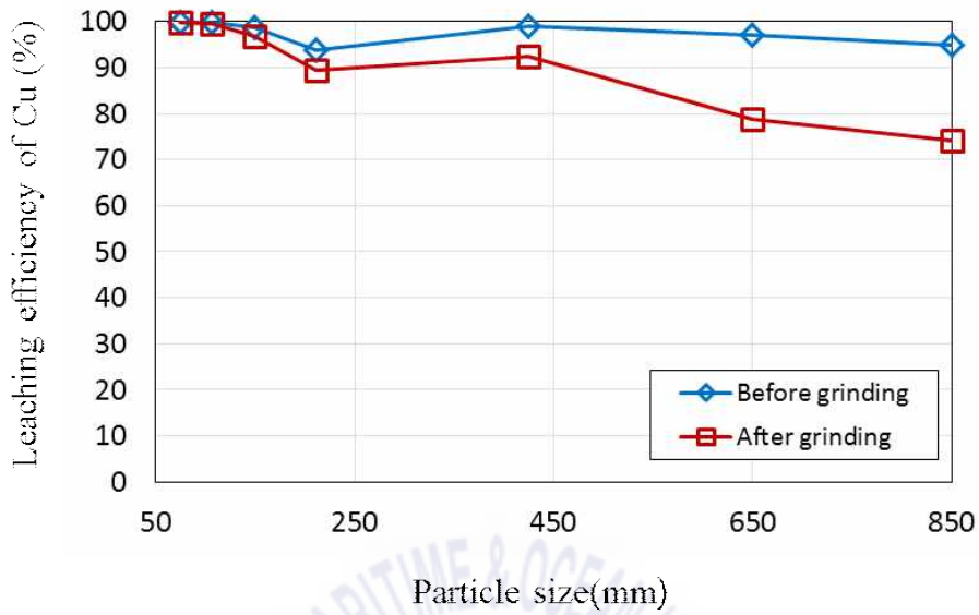
Fig. 23 Leaching efficiency compared to the results before and after ball mill grinding
