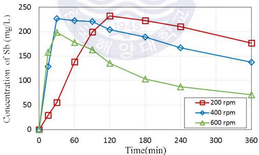
Fig. 30 Effect of agitation speed with O_2 on the concentration of Sb from Cu speiss
