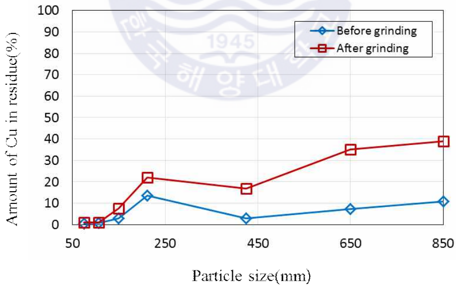
Fig. 24 Amount of Cu in residue compared to the results before and after ball mill grinding
