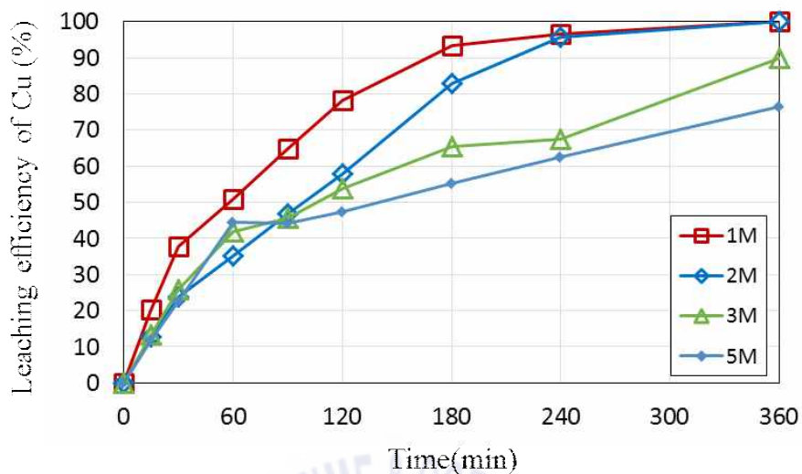
Fig. 32 Effect of HCl concentration on the leaching of Cu from Cu speiss
