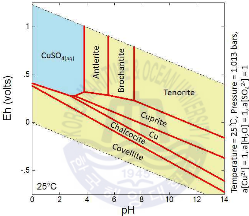
Fig. 8 Eh-pH diagram for Cu-SO 4 2- -H 2 O system (박일환, 2016)
