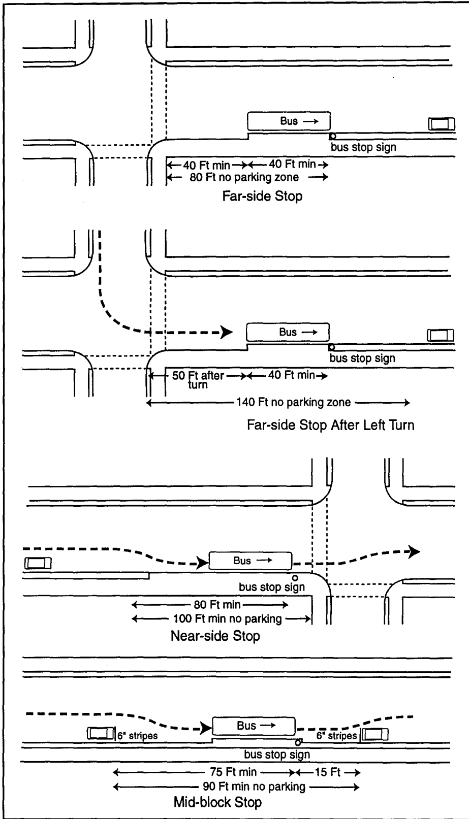
Recommended Bus Stop/Zone Placement Figure 33
