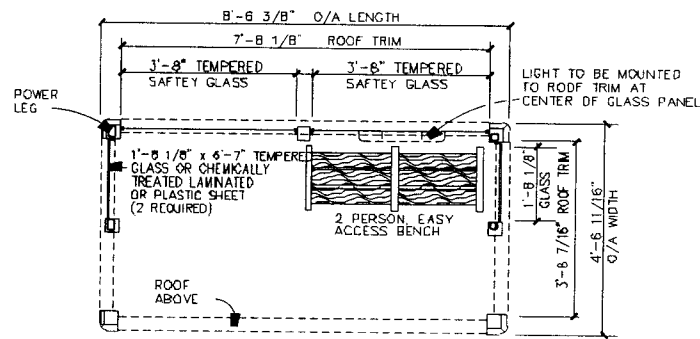
TOP VIEW - ROOF REMOVED
