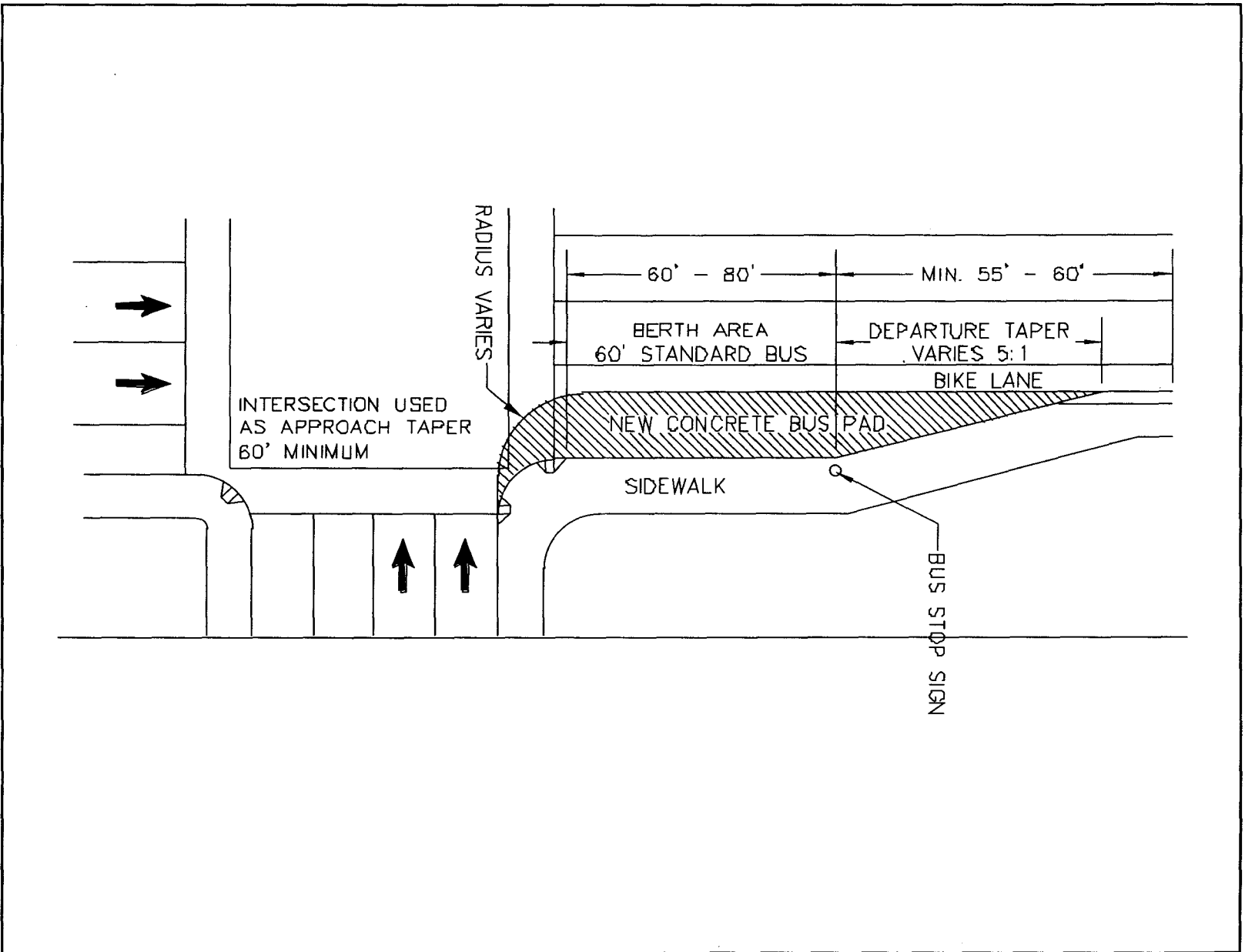
Bus Pull Out & Bus Pad Figure 29
