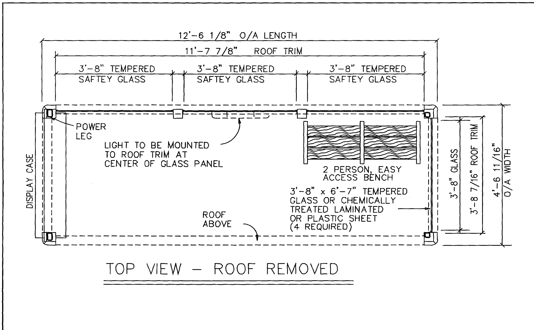
TType "BX" Shelter Without Display Figure 10
