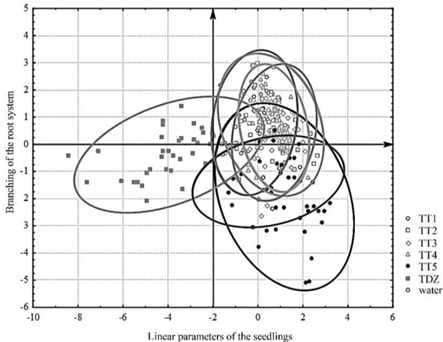
Figure 5. Visualisation of discriminant analysis results.
