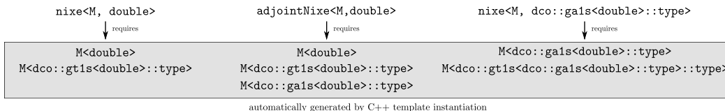
Figure 3: Instantiation graph for nixe and adjointNixe , the top-level subroutines of NIXE for simulation and modified discrete adjoint sensitivity analysis, respectively. M is the model class template described in Section 4. For a description of dco/c++ data types see Section 3.
