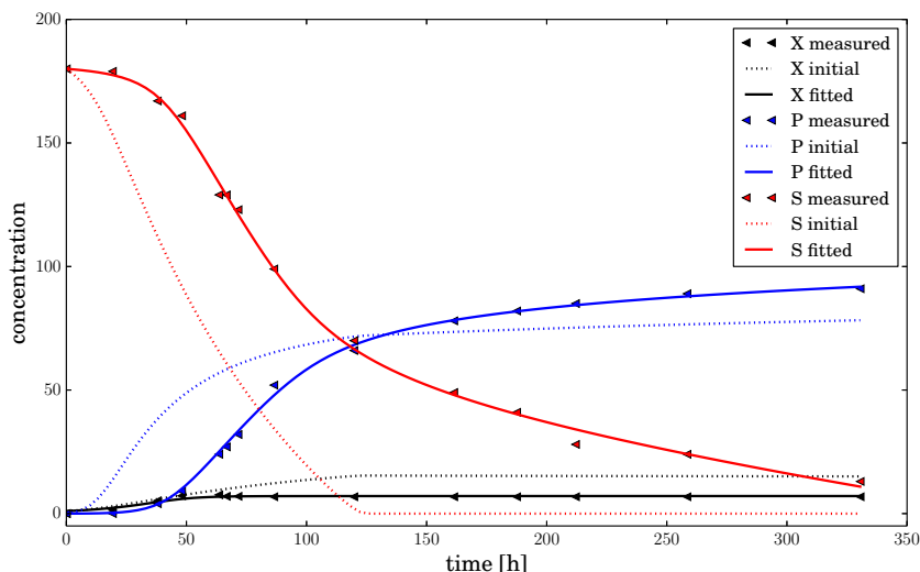
Figure 5: Measurements and simulated temporal evolution of the concentrations of the components mass of A. terreus (X), product (P), and substrate (S).
