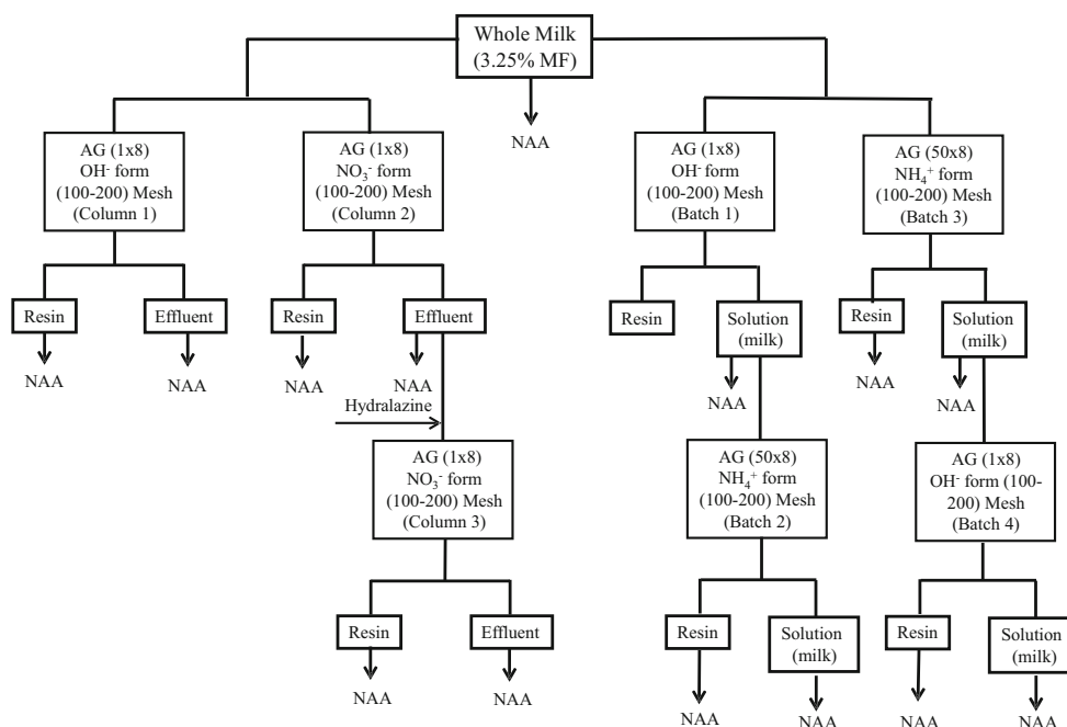
Fig. 2 Scheme for the separation of anionic and cationic iodine fractions in milk
