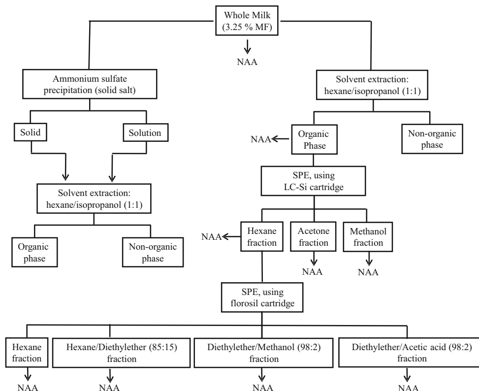
Fig. 1 Fractionation scheme for halogens bound to milk lipids
