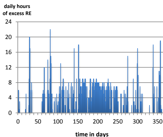
Figure 2 Daily hours of expected excess electricity from RE in the year 2020 in Germany
