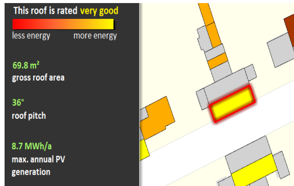
Figure 1 Solar potential for the modelled house from “Solar Atlas” (Stadt Bottrop, 2014)
