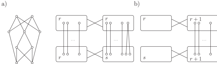
Figure 3.4: Graphs of Example 3.18 showing the tightness of Theorem 3.17.
