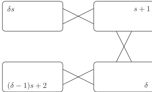
Figure 3.2: Graphs showing the tightness of Theorem 3.11.
