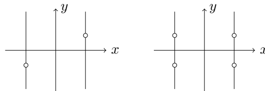
Figure 2.4: The solutions of S in Example 2.60 on the left and of S' on the right.
