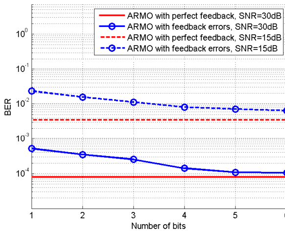
Fig. 4. BER performance vs. different number of bits for feedback quantization, P_e = 10^{-3}
