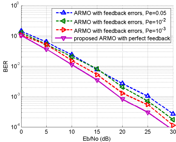
Fig. 3. BER performance for ARMO algorithm with perfect and imperfect feedback links with different P_e , quantization bits = 4
