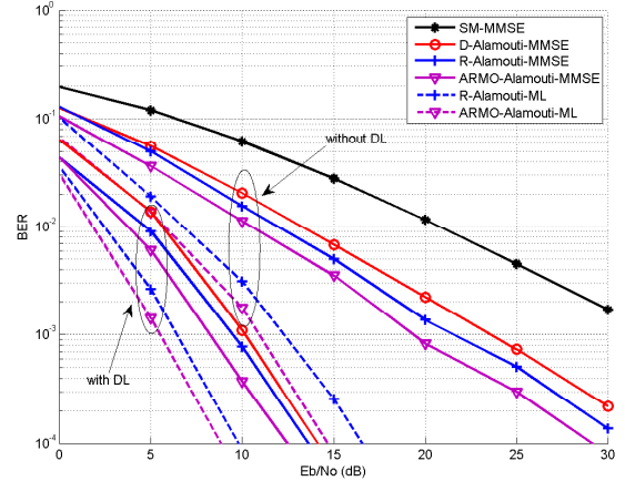
Fig. 2. BER performance vs. E_b/N_0 for ARMO Algorithm with and without the direct link
