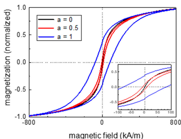
Figure 6. Normalized minor loops of pure magnetite ( a = 0 ) and particles with a Co content of 12.5% ( a = 0.5 ) as well as 25% ( a = 1 ) recorded at room temperature confirm a significant increase in the coercivity for increasing Co content of the particles. The inset depicts a higher magnification of the hysteresis curves at low magnetic field strengths.
