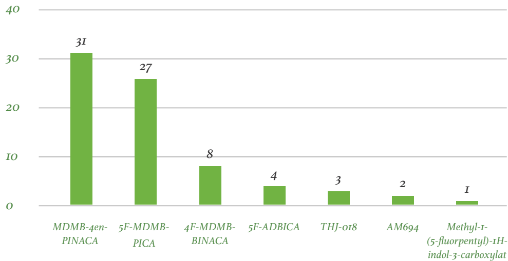
Figure 1: Synthetic cannabinoids analysed by frequency in the 50 samples of occurrence.
