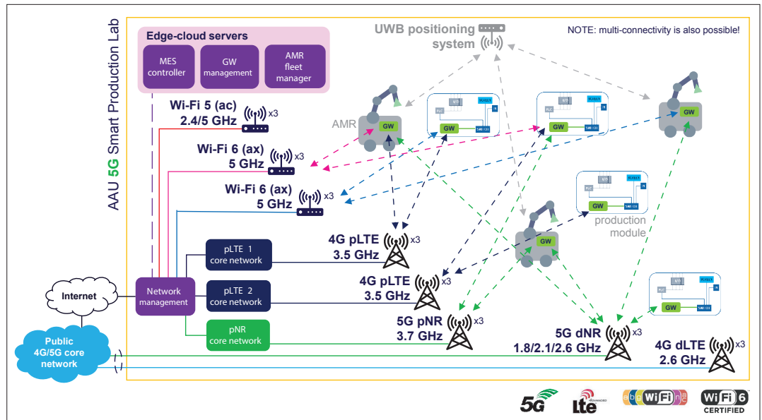
FIGURE 1. High-level overview of the Industry 4.0 wireless production testbed deployed at AAU, illustrating the swarm production concept with production modules and AMRs distributed over the production facilities, and the dedicated network infrastructure available for the testing of industrial use cases.
