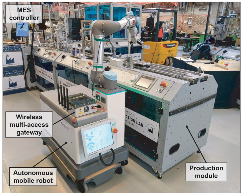
FIGURE 2. Picture of some of the industrial machinery elements of the testbed, including the FESTO CP Factory production line in its standard wired configuration and one of the Mir200-based AMRs. The picture also depicts one of the wireless multi-access gateways used in the various experiments to interface the industrial equipment to the different networks.
