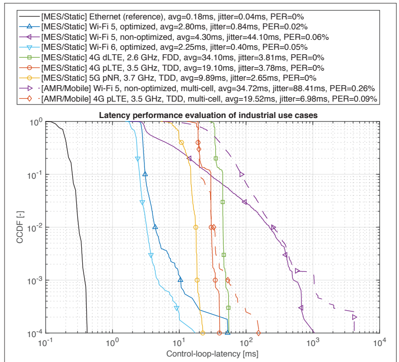
FIGURE 3. Wireless performance results for the wireless control of industrial production (MES/static) and for the control of AMRs (AMR/mobile) industrial use cases over different communication technologies.
