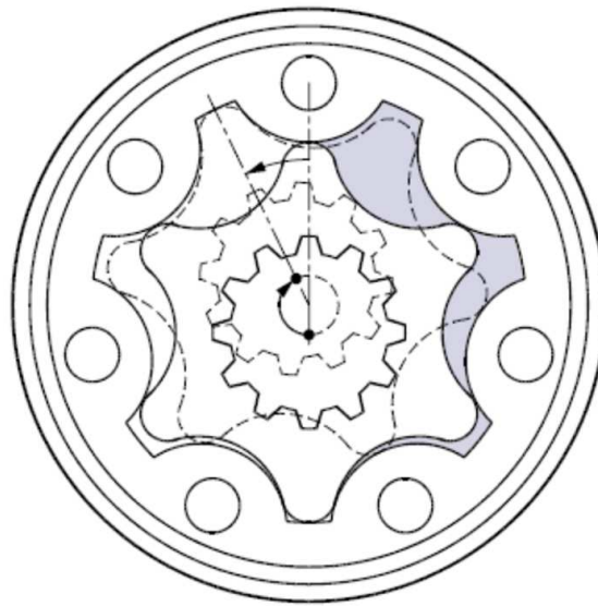
Figure 1: Illustration of an orbital gear-set from a technical brochure (Danfoss A/S 2015: 8). Eccentricity between the gear-wheel and gear-rim enable the orbital movement for which the principle is named.
