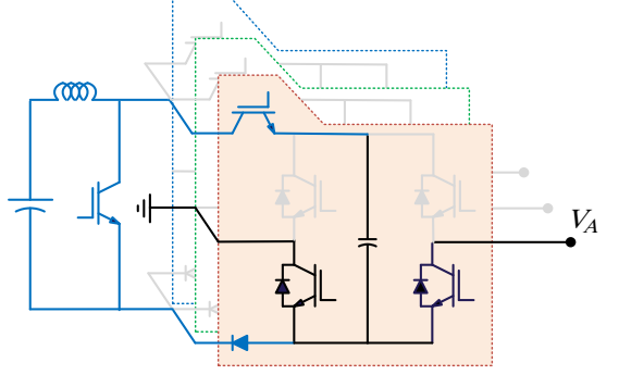
(b) Zero voltage level [O]
