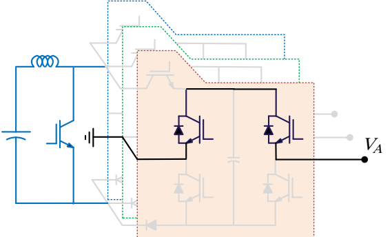
(c) Zero voltage level [O]
