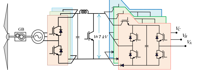
Fig. 4. Proposed SSFB-TPI in a medium voltage application.
