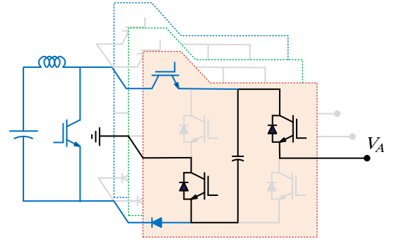
(a) Positive voltage level [P]
