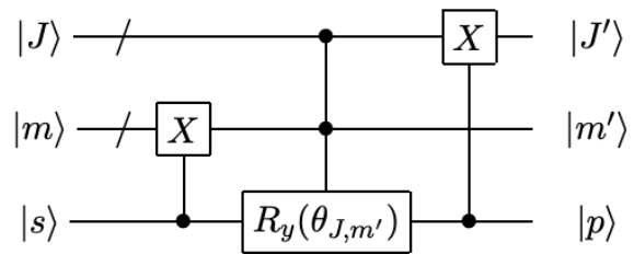
FIG. 4: Schematic description of the Clebsch-Gordan transformation by Bacon, Chuang, and Harrow [14]. Here s represents a single qubit which is added to a system with angular momentum J and m . On the right, J' and m' label the resulting angular momenta, and p keeps track of the pathway through which those values are obtained. The slash denotes a wire containing a register of qubits, the control-X gate adds angular momentum appropriately, and the controlled rotations (one for each J, m' ) produce the correct amplitudes.
