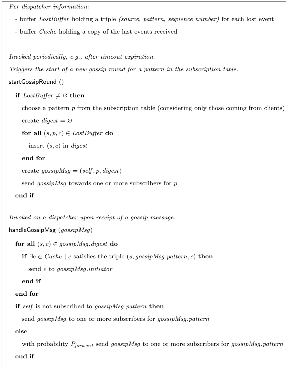
Figure 5.3: Pull algorithm.
