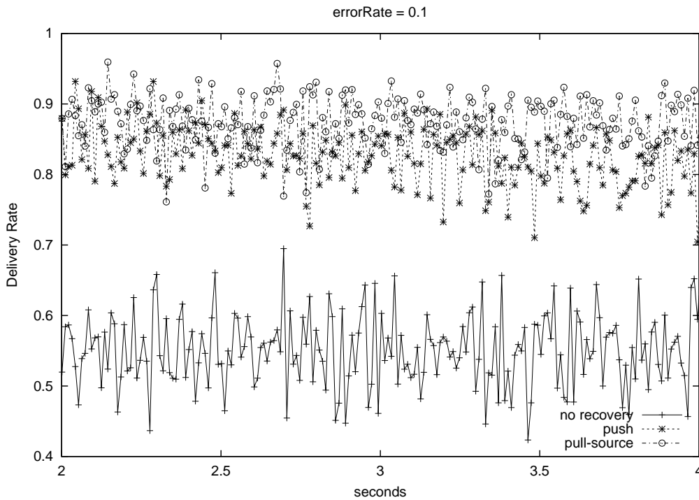
Figure 6.1: Example of delivery in a very critical scenario
