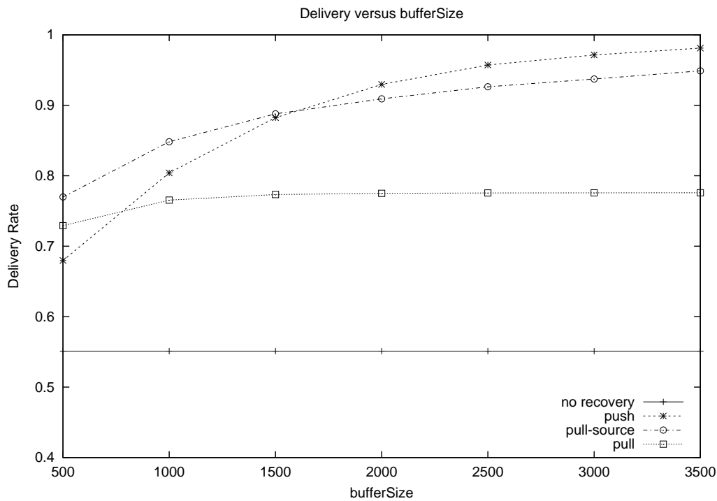
Figure 6.5: Effect of bufferSize on delivery rate
