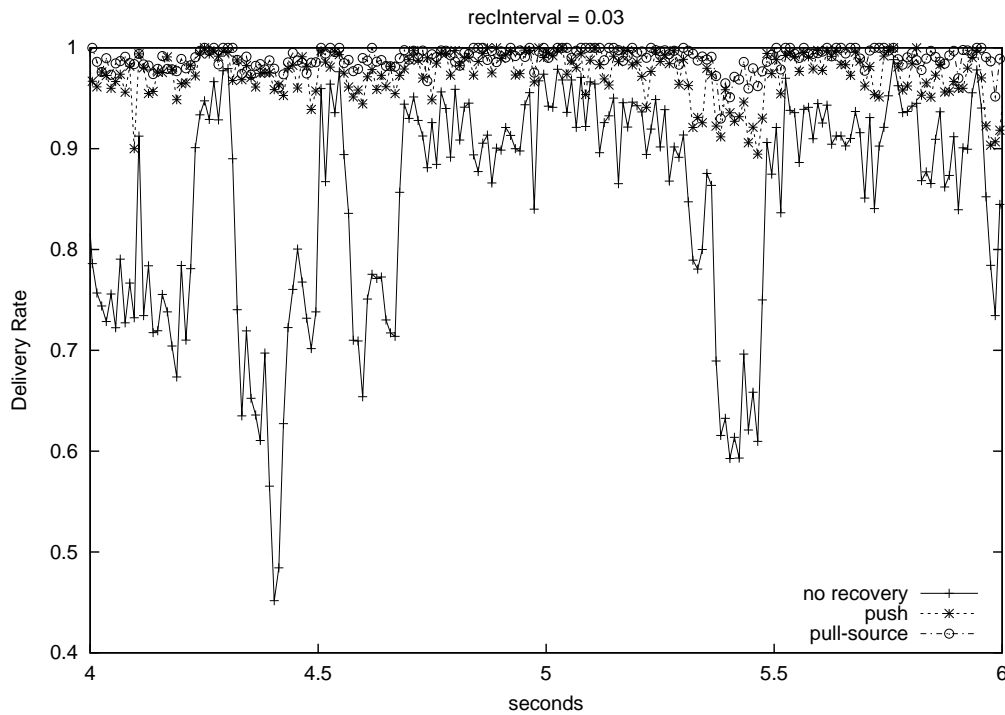
Figure 6.3: Example of delivery in a scenario with overlapping reconfigurations
