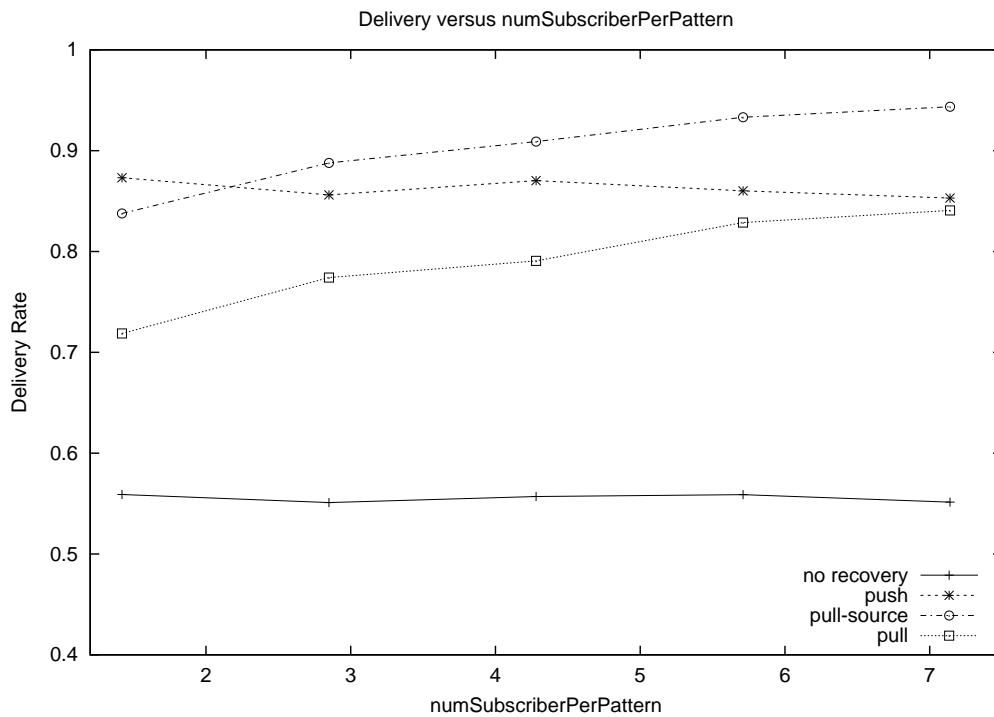
Figure 6.7: Performance in different content-based scenarios (II)
