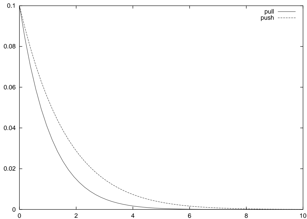
Figure 3.3: The convergence of push and pull approach
