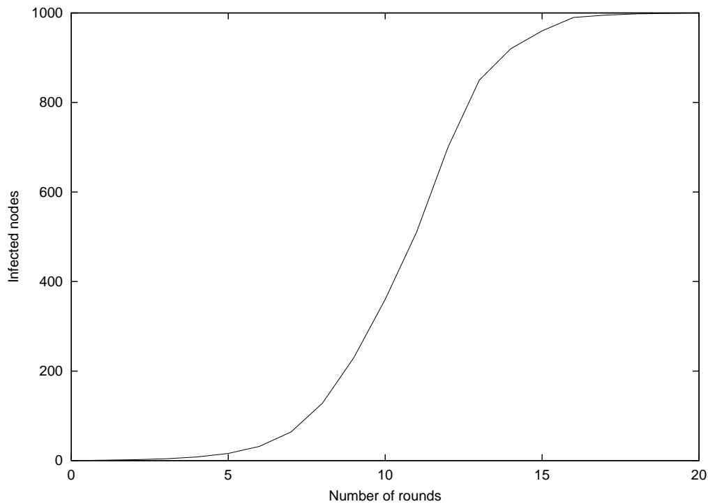
Figure 3.1: An example of the diffusion of an infection in a finite population.
