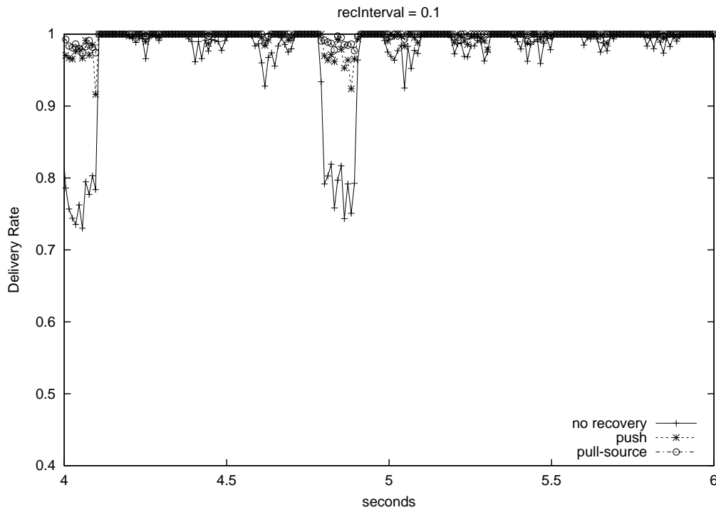
Figure 6.4: Example of delivery in a scenario with non-overlapping reconfigurations
