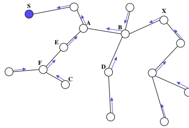
Figure 2.3: A undirected acyclic graph with subscriptions laid down according to a subscription forwarding scheme.
