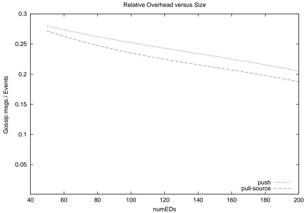
Figure 6.10: Percentage of traffic due to the gossip messages as the system size grows
