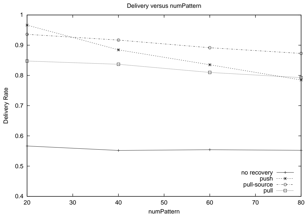
Figure 6.6: Performance in different content-based scenarios (I)
