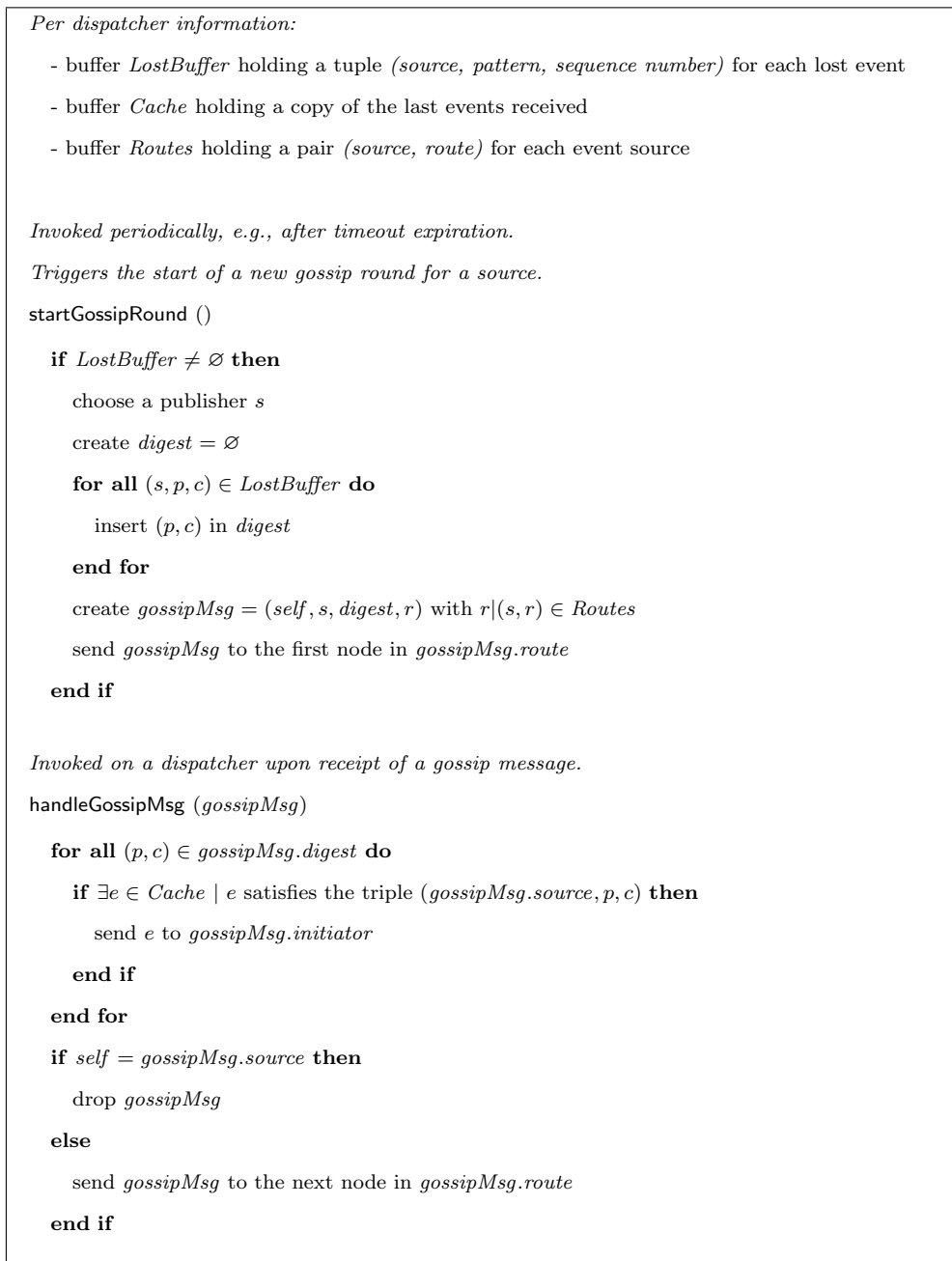
Figure 5.4: Source-based algorithm.
