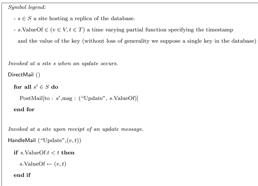
Figure 3.4: Direct mail algorithm.
