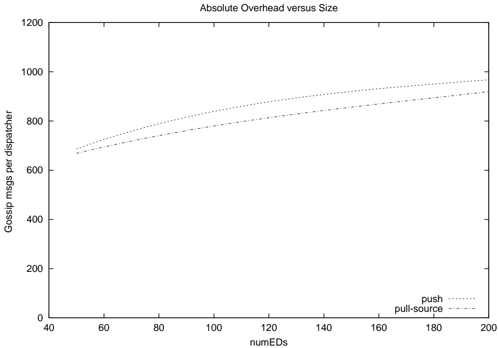
Figure 6.9: Measurement of gossip traffic per dispatcher as system size grows
