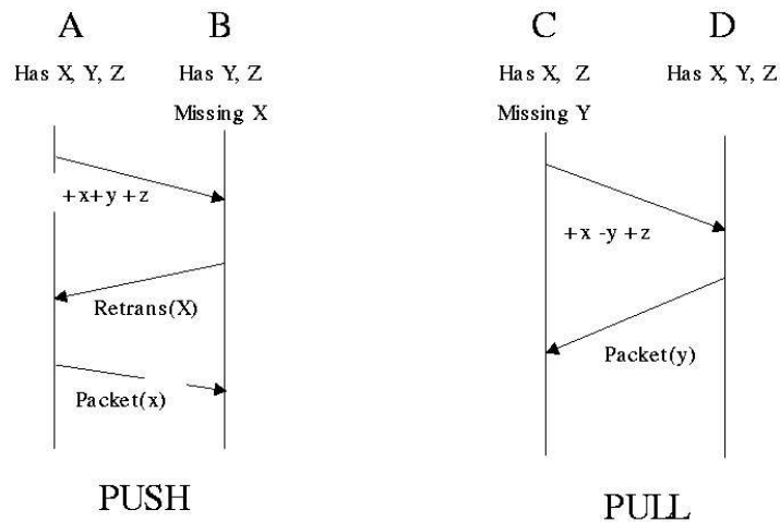
Figure 3.2: Gossip recovery examples: in (PUSH) gossipier \mathcal{A} pushes out a missing packet \mathcal{X} to \mathcal{B} . In (PULL) gossipier \mathcal{C} pulls in a missing packet \mathcal{Y} from \mathcal{D}
