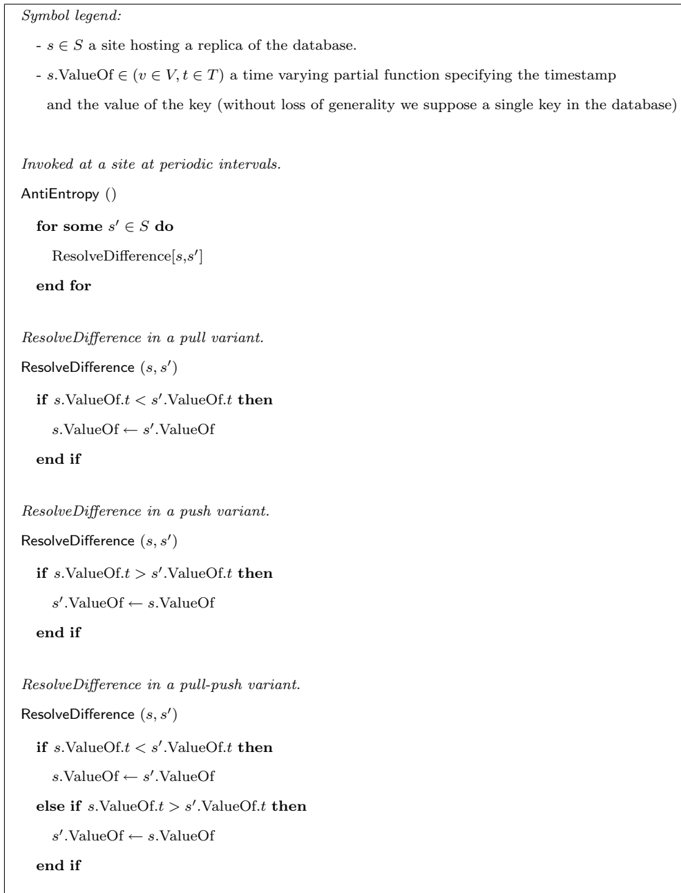
Figure 3.5: Anti-entropy algorithm.
