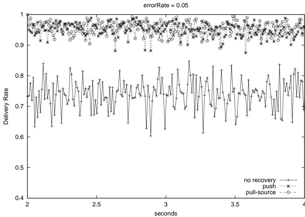
Figure 6.2: Example of delivery in a lossy scenario
