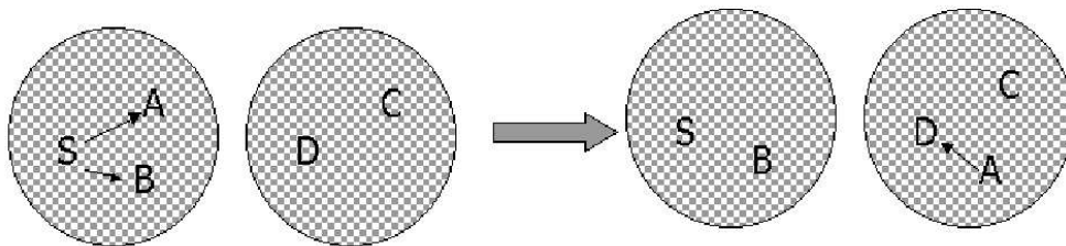
Figure 3.8: An example of message delivery in presence of network partition
