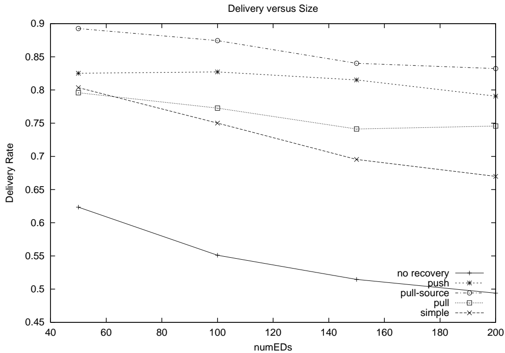
Figure 6.8: Effect of size on delivery rate
