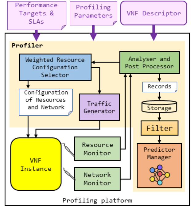
Fig. 2: High-Level architecture of our proposed NAP method including the main building blocks
