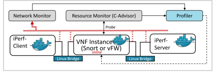
Fig. 5: Experiment Setup
