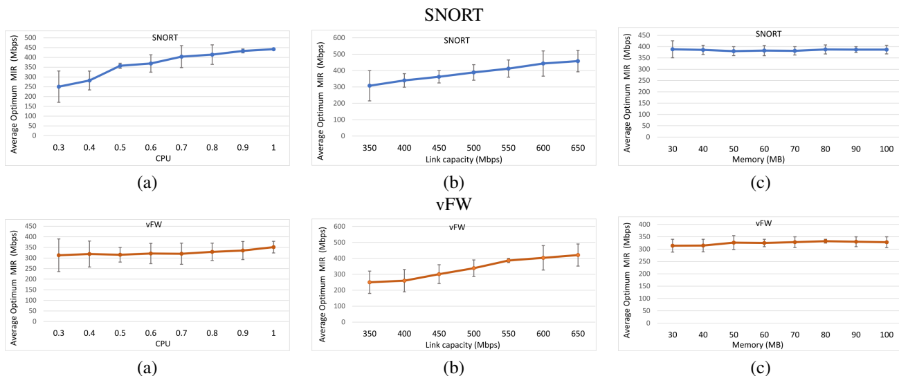
Fig. 7: The Correlation between (a) CPU, (b) Link Capacity, (c) Memory, and the Optimum MIR per SNORT and vFW, respectively. Results are annotated with 95% confidence intervals.
