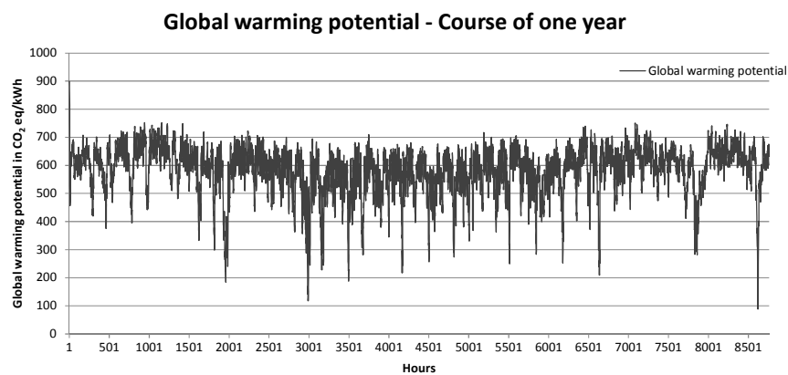
Fig.1: Course of the global warming potential of the energy mix in Germany during one year
