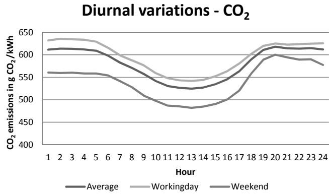
Fig.2: Diurnal variation of the CO 2 eq emissions of the energy mix for one day
