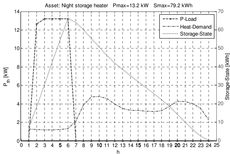
Fig.5: Operating behavior of night storage heaters for a winter day
