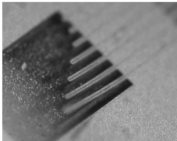
Fig. 2. Set of Cantilever beams with length from 50 \mu\text{m} to 1000 \mu\text{m} and 50 \mu\text{m} in width.
