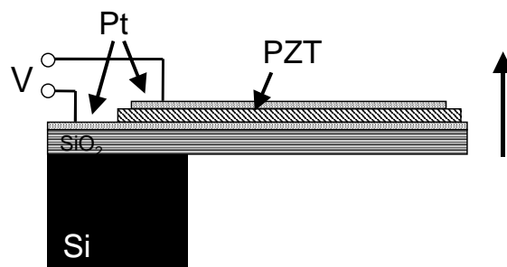
Fig. 1. Schematic concept of a PZT actuated cantilever.
