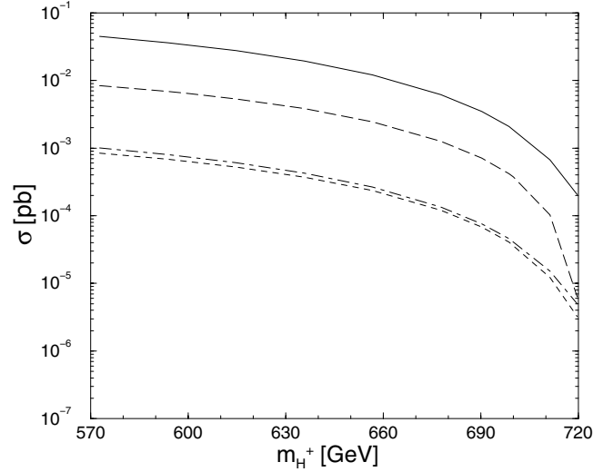
Figure 2: The cross sections for \gamma\gamma \rightarrow A^0 \rightarrow H^\pm W^\mp . m_{A^0} = 800 GeV, \sqrt{s_{ee}} = 1000 GeV. The solid (dashed, dotted and dat-dashed) curve indicates the case for \tan \beta = 1.5 (7, 30 and 40).
