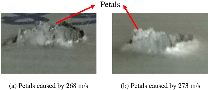
Figure 10: Petals developed on the rear plate
