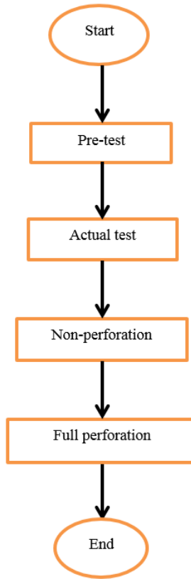
Figure 4: Methodology flow-chart
