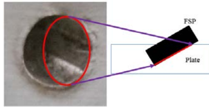
Figure 5: The crater developed after impacted by FSP with initial velocity of 237 m/s
