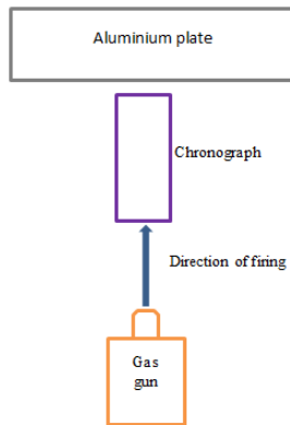
Figure 2: Schematic drawing of test set-up
