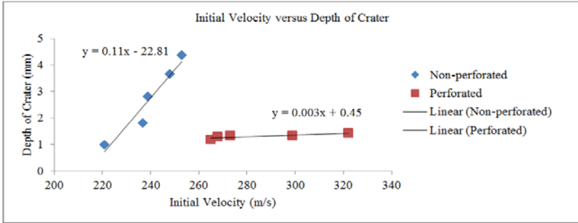
Figure 11: Correlation between the initial velocity and depth of crater for both cases
