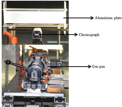
Figure 1: Actual picture of test set-up
