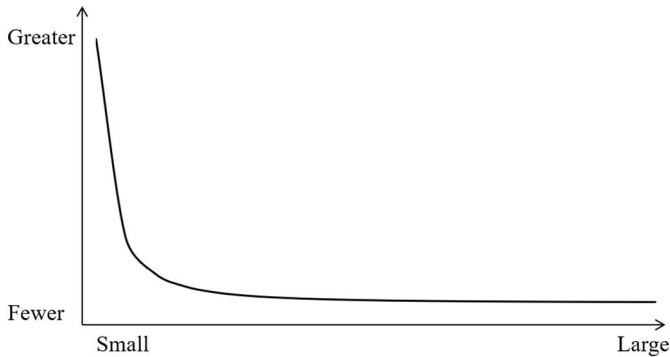
Figure 2 The asymptotic, long-tail curve of a power-law distribution
