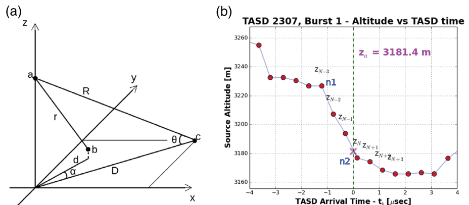
Figure A1. Methods information. (a) Source-centric coordinate system for temporal correlations. The TGF source is at (x_a, y_a, z_a) , with the plan x, y location serving as the coordinate origin. The TASD station is at location b relative to the origin and the reference altitude, and the INTF/FA is at the more distant location c . (b) Iteration at 0.5 \mu\text{s} time steps used in the alternative approach for determining the source altitude (TGF A in this case), showing the occurrence of enhanced-speed downward FNB immediately before the TGF onset (red “x”).
