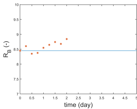
Figure 14: Calculated and measured receptor of anti-inflammatory cytokine R_B fluorescence versus time, markers indicate measured data, simulation results are shown as lines.
