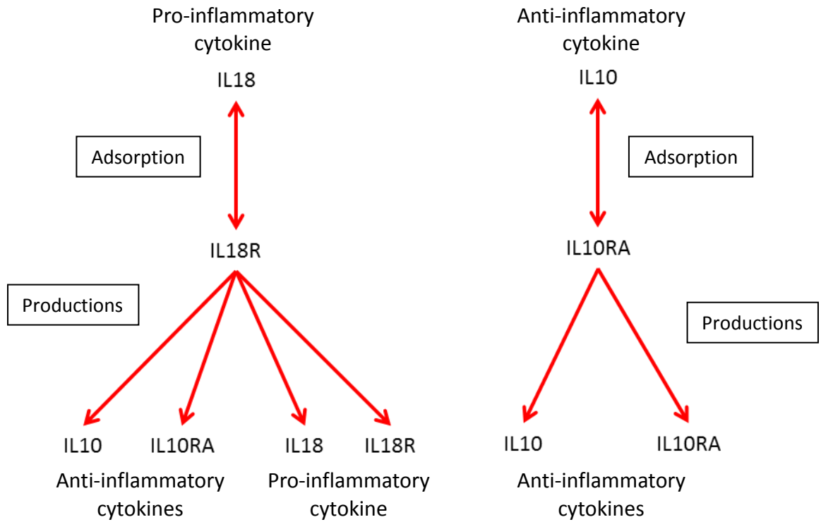
iv) Figure 2 : Schematic representation of adsorption and production mechanisms related to IL18 and IL10 cytokines
