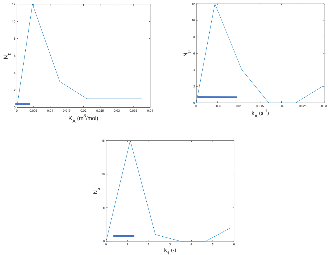
Figure 8: Parameter value distributions by number of patients for K_A , k_A , k_1 and the intervals corresponding to all dead patients.
