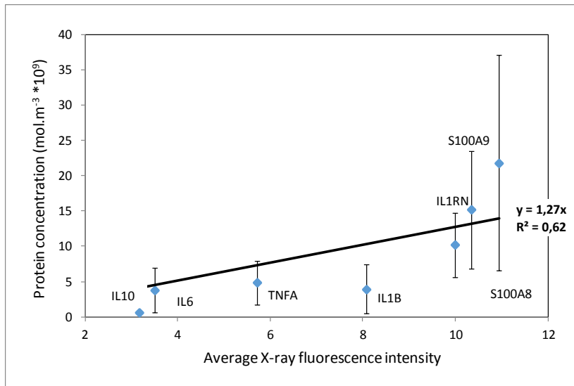
Figure 3: Calibration curve for protein concentration from Average X-ray fluorescence values in healthy patients
