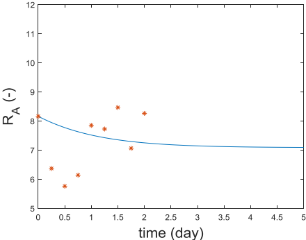
Figure 12: Calculated and measured receptor of pro-inflammatory cytokine R_A fluorescence versus time, markers indicate measured data, simulation results are shown as lines.
