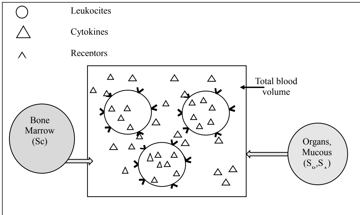
Figure 4: Representation of the blood system
