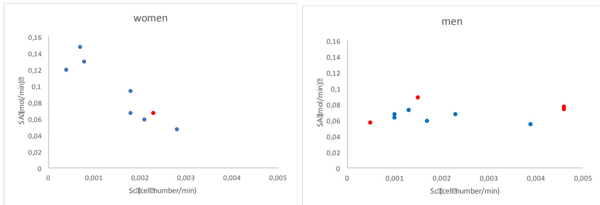
Figure 9: Cytokine source terms, S_A and S_B , relative to cell source term, S_C . Red dots indicate deceased patients and blue dots represent survivors.
