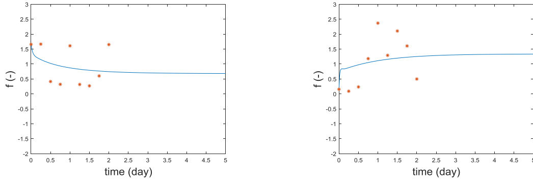
Figure 16: calculated and measured inflammation level function f versus time, markers indicate measured data, simulation results are shown as lines.
