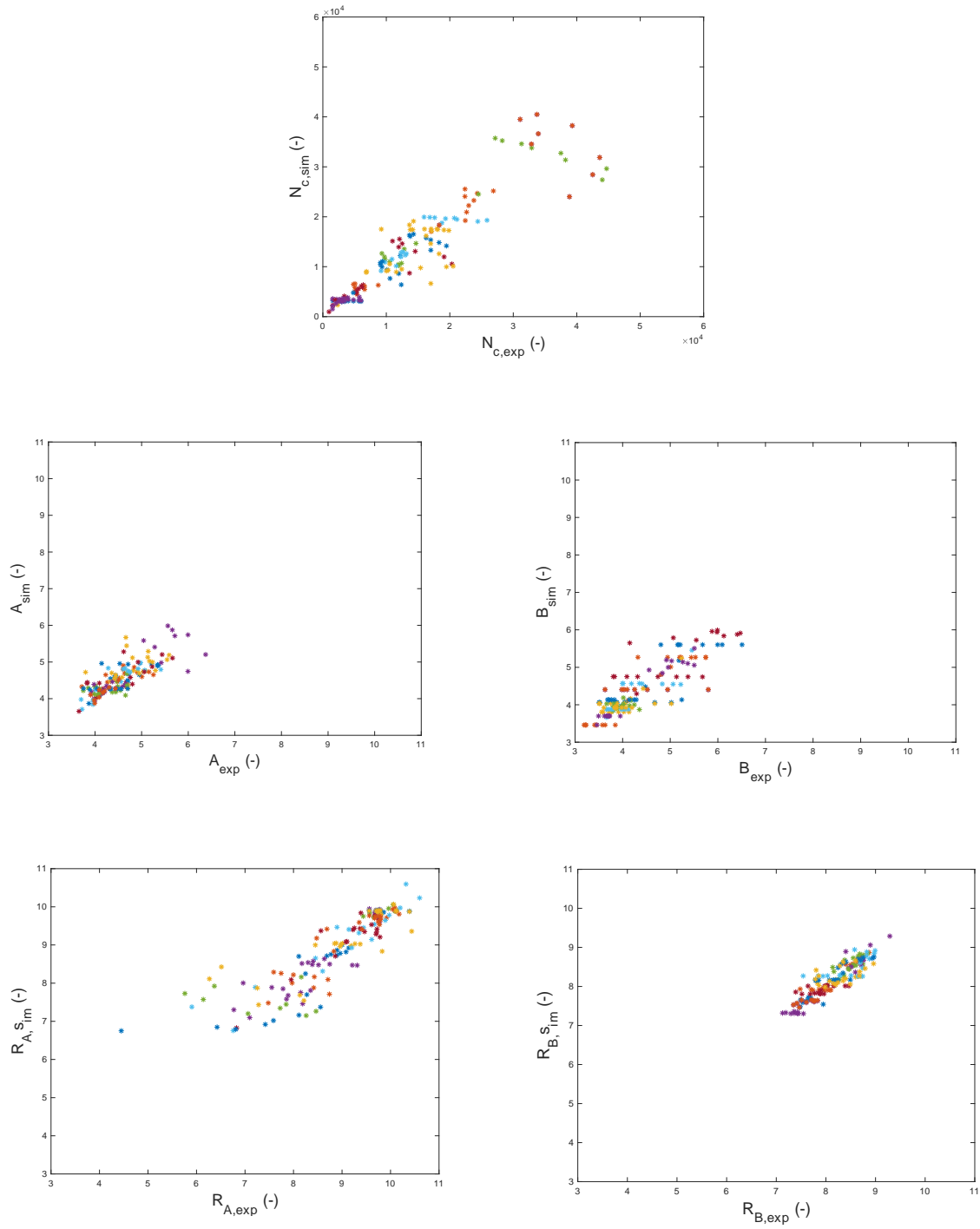
Figure 10: Parity plots for calculated N_c , A , B , R_A , R_B fluorescence against measured data (each color corresponds to one patient). Pearson's correlation coefficient values are 0.906 for N_c , 0.715 for A , 0.818 for B , 0.855 for R_A and 0.874 for R_B .
