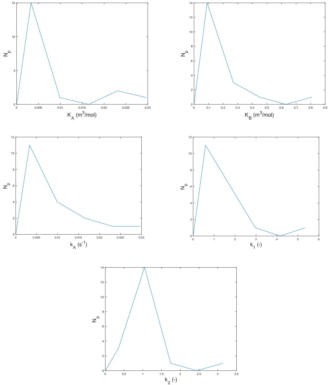
Figure 7: Parameter value distributions by number of patients for K_A , K_B , k_A , k_1 , k_2 .
