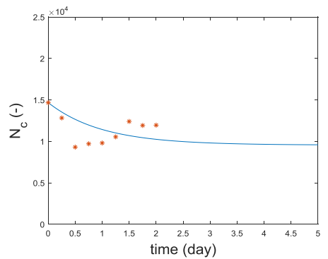
Figure 15: Calculated and measured cell number N_c versus time, markers indicate measured data, simulation results are shown as lines.
