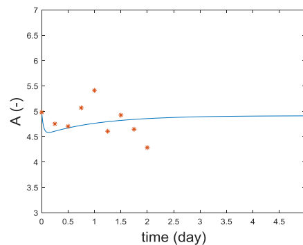
Figure 11: Calculated and measured pro-inflammatory cytokine A fluorescence versus time, markers indicate measured data, simulation results are shown as lines.
