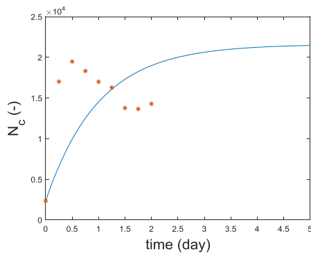
Figure 15: Calculated and measured cell number N_c versus time, markers indicate measured data, simulation results are shown as lines.
