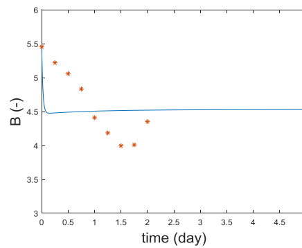
Figure 13: Calculated and measured anti-inflammatory cytokine B fluorescence versus time, markers indicate measured data, simulation results are shown as lines the anti-inflammatory cytokine. As mentioned earlier, the model was not very sensitive to the parameters for the anti-inflammatory cytokine and here we observe that, despite apparent trends in the data, the model did not pick up this dynamic but rapidly adjusted to a value close to the mean.
