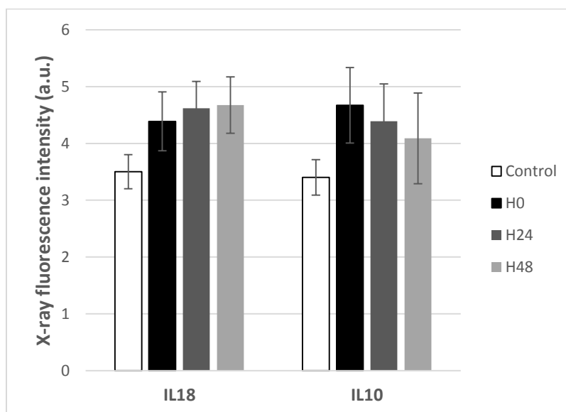
Figure 1: Mean X-ray fluorescence signal measured for IL18 and IL10 cytokines at 0, 24h and 48h after septic shock. The corresponding signals obtained for the healthy volunteers are also 7
