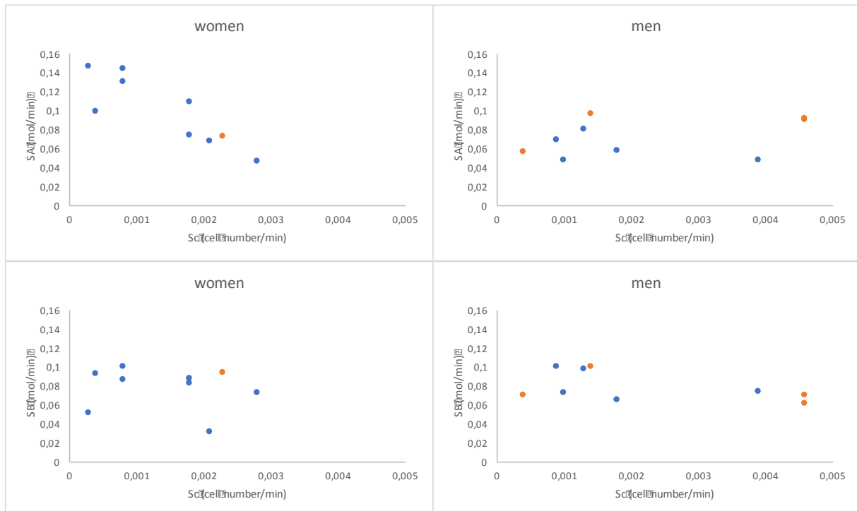
Figure 6: Cytokine source terms, S_A and S_B , relative to cell source term, S_C . Red dots indicate deceased patients and blue dots represent survivors.
