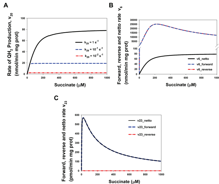
FIGURE 5 | Computer simulated bell-shaped vs. hyperbolic kinetics of ROS production and succinate-Q reductase (SQR) activity of CII. (A) The hyperbolic stationary dependence of the QH 2 production rate, v_{20} , on the succinate concentration in the basal state ( k_{29} = 1 \text{ s}^{-1} ) and upon intermediate ( k_{29} = 0.1 \text{ s}^{-1} ) and strong ( k_{29} = 0.01 \text{ s}^{-1} ) inhibition of respiratory Complex III (CIII) that was simulated by decreasing the catalytic constant k_{29} of QH 2 oxidation. (B) Computer simulated dependence of stationary rates of unidirectional mainstream electron flows in forward (from FADH 2 to oxidized [2Fe-2S] cluster), v_{6\_forward} , and reverse (from reduced [2Fe-2S] cluster to FADH 2 ), v_{6\_reverse} , direction and netto rate v_{6\_netto} = v_{6\_forward} - v_{6\_reverse} on the succinate concentration. (C) Computer simulated dependence of stationary rates of unidirectional bypass electron flows in forward (from FADH 2 to O 2 ), v_{23\_forward} , and reverse (from O 2 - to FADH 2 ), v_{23\_reverse} , direction and netto rate v_{23\_netto} = v_{23\_forward} - v_{23\_reverse} on the succinate concentration. Values of the rate constant k_{29} shown in Figure 3A . Black solid curve corresponds to the k_{29} = 1 \text{ s}^{-1} , blue dashed curves – k_{29} = 0.1 \text{ s}^{-1} , and red dash-dot curves – k_{29} = 0.01 \text{ s}^{-1} . The rest model parameter values are presented in Supplementary Table S2 . Curves in Figures 3B,C are designated as follows: black solid curves correspond to the netto rates v_{6\_netto} ( B ) and v_{23\_netto} ( C ), blue dashed curves – unidirectional forward rates v_{6\_forward} ( B ) and v_{23\_forward} ( C ), and red dash-dot curves – unidirectional reverse rates v_{6\_reverse} ( B ) and v_{23\_reverse} ( C ). All computer simulations were made at model parameter values presented in Supplementary Table S2 .
