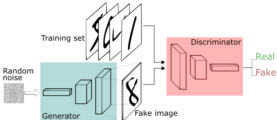
Figure 5.8: The training procedure for the simplest GAN algorithm as described in Goodfellow et al. (2014) for the MNIST dataset. Image from sthalles.github.io (2020) .
