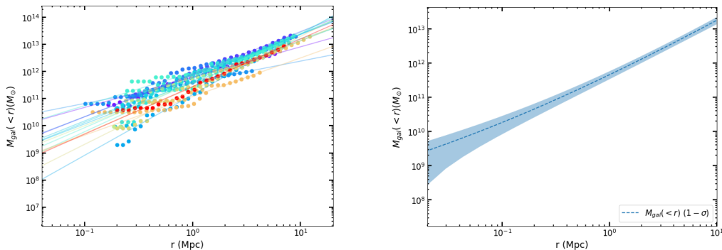
Figure 4.6: Results for the galaxy mass distribution of the 58 cluster stack. The result on the left contains galaxy masses M_{gal}(< r) at different r for each cluster in the stack along with the extrapolated best-fit lines to bring the measurements to the same scale. The figure on the right shows the mean and the standard deviation of the cluster stack galaxy masses.
