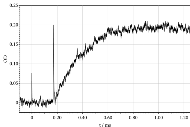
Fig. 5 The same as Fig. 4, but at lower temperature ( T = 1246 K, [\text{Ar}] = 4.8 \times 10^{-5} mol \text{cm}^{-3} ; 209 ppm (\text{C}_2\text{F}_5)_3\text{N} in Ar; \varepsilon(1246 \text{ K})/\varepsilon(1347 \text{ K}) \approx 1.15^{13} ).
