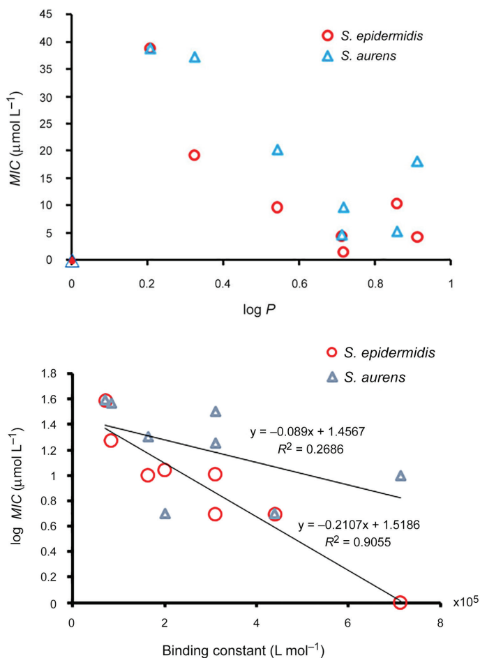
Fig. 7. a) A plot of MIC values of different products between their measured \log P values. b) A plot of MIC between the binding constants of the products. Each point in the plot represents a different product.
