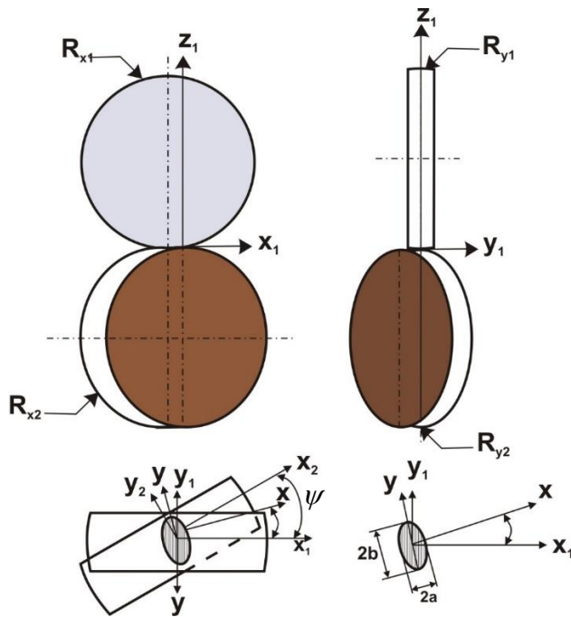
Figure 4.2: Wheel and rail roller with the yaw angle adjusted on the rail roller
