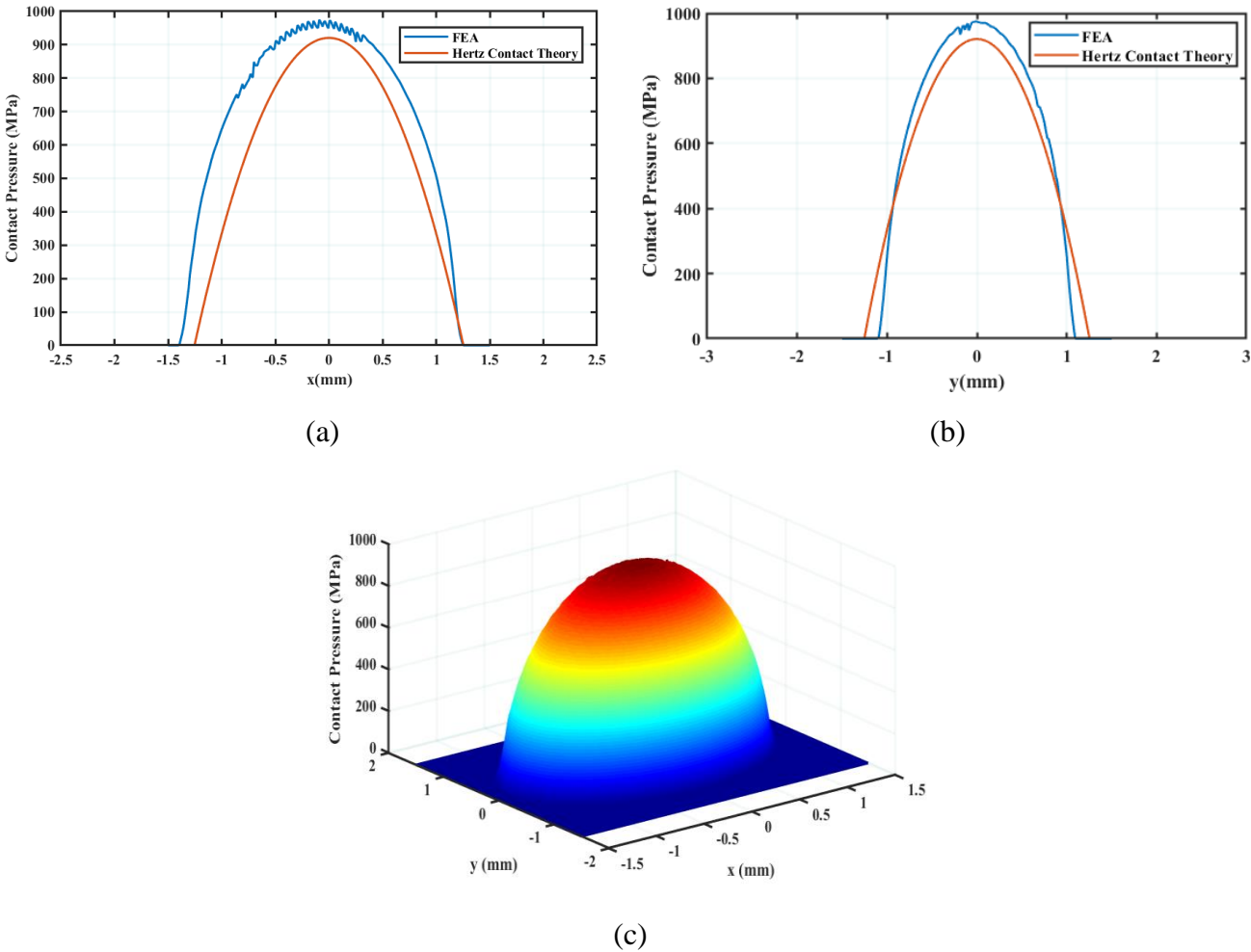
Figure 4.6: Normal contact pressure developed the contact area for normal applied load of 2500N (a) Lateral direction (b) Longitudinal direction (c) 3D plot of the contact pressure obtained from FEA.
