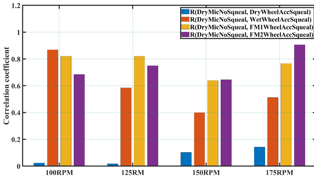
Figure 7.1: Correlation method applied to the skewness feature values from the microphone and wheel accelerometer data.
