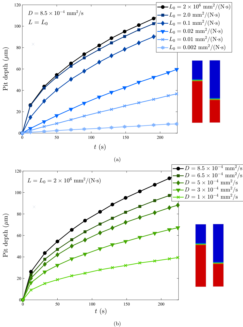
Figure 6: Pencil electrode test. Pit depth versus time t as a function of (a) the interface kinetics coefficient L = L_0 , and (b) the diffusion coefficient D .
