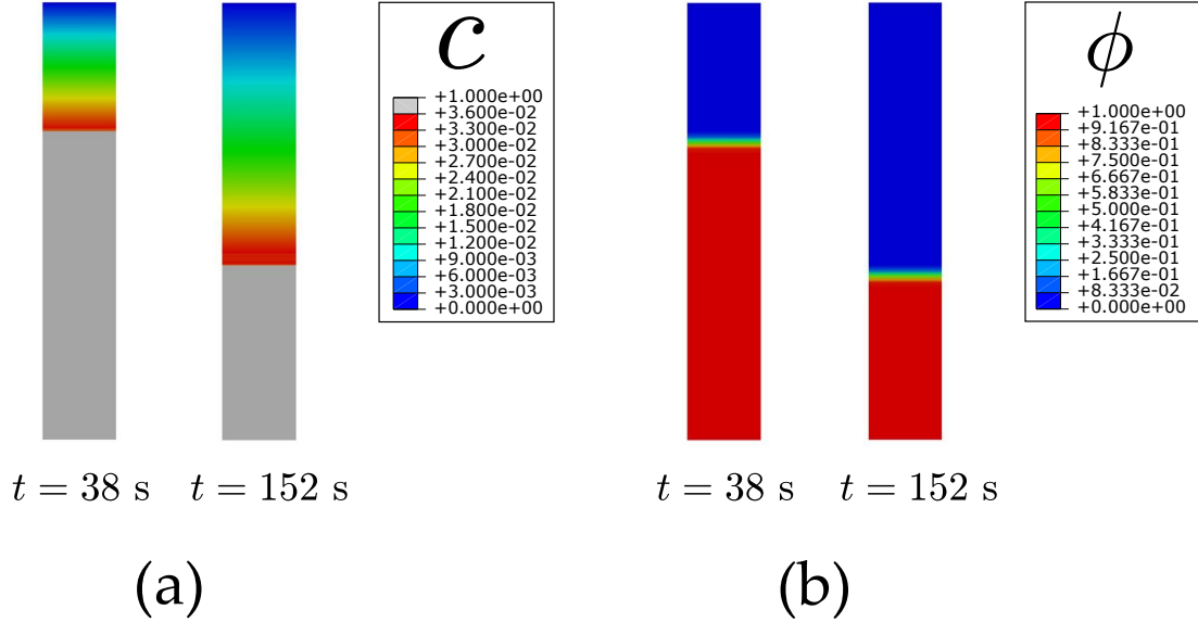
Figure 4: Pencil electrode test. Contours of (a) normalised concentration and (b) phase field at times t = 38 \text{ s} and t = 152 \text{ s} .
