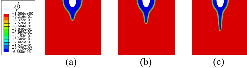
Figure 13: SCC from a semi-elliptical pit. Contours of the phase field after t = 900 s for a remote displacement of u^\infty = 0.1 \mu\text{m} and three selected values of the film stability parameter: (a) k = 2 \times 10^{-4} , (b) k = 5 \times 10^{-4} , and (c) k = 1 \times 10^{-3} .
