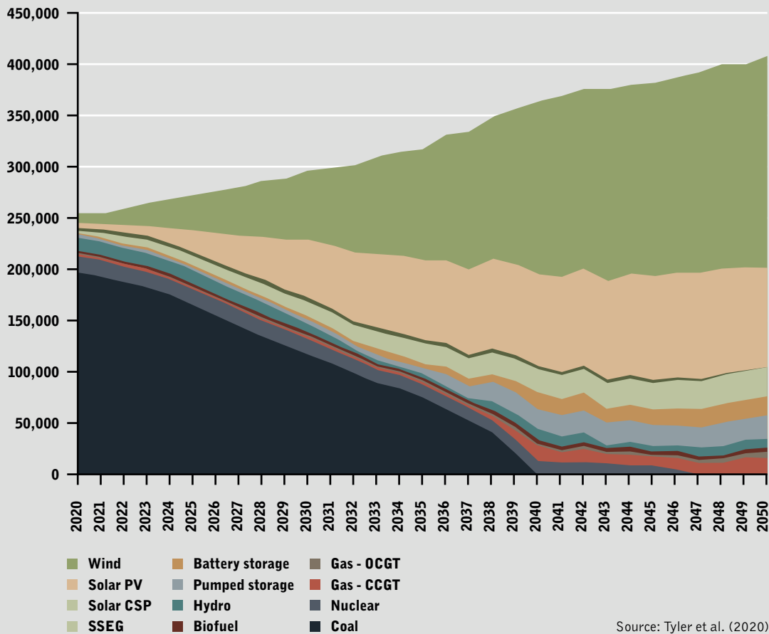
Fig. 5: Renewable energy build scenario to achieve coal phase down by 2040
