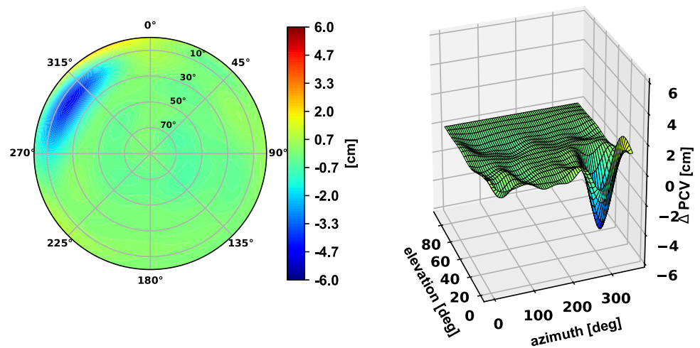
Fig. 5 Example of L1 PCV difference between a single calibration and the type mean. Polar and 3D plot with respect to azimuth and elevation are reported
