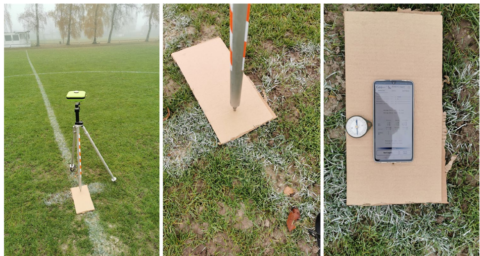
Fig. 8 Soccer field setup. Left and middle panel: the geodetic receiver has been used to compute the correct reference position of the smartphone. Right panel: the Mate20X has been aligned to geographic north, with the bottom edge eccentric over the reference point (the hole in the piece of cardboard)
