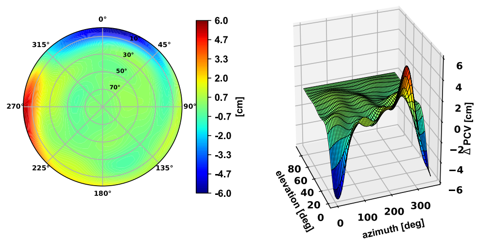
Fig. 6 Example of L5 PCV difference between a single calibration and the type mean. Polar and 3D plot with respect to azimuth and elevation are reported
