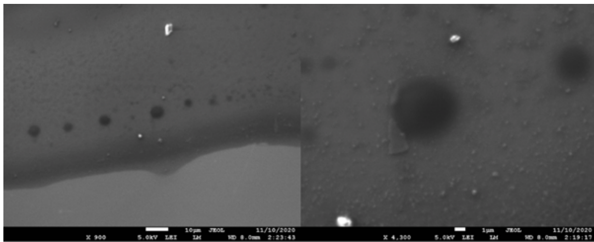
FIG. 9. Graphite aggregates in inkjet-printed graphene
