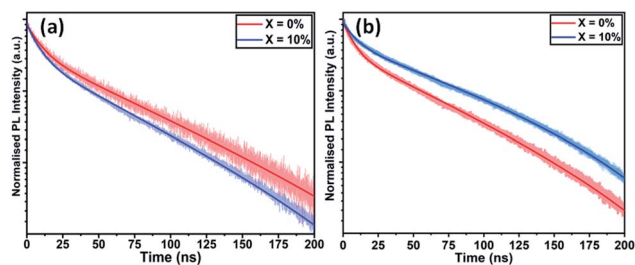
Fig. 4 Time-resolved photoluminescence of triple-cation perovskite films with KI added at 0% and 10% cast on (a) ITO/ \text{SnO}_2 and (b) FTO/ \text{SnO}_2 .
