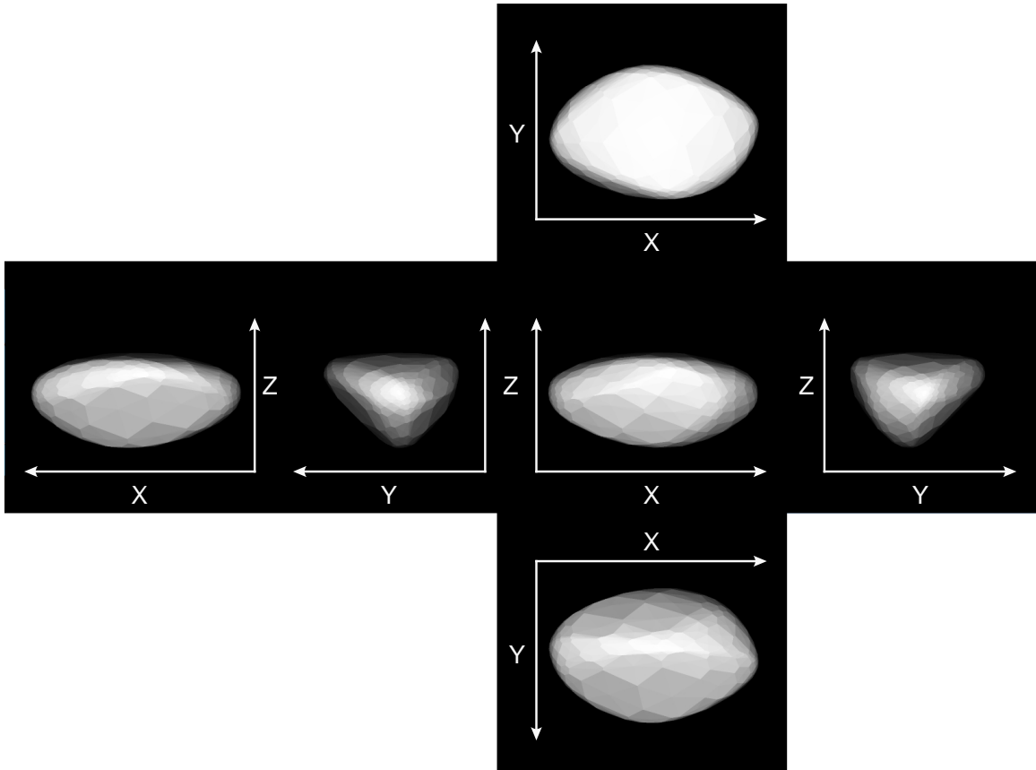
Figure 6. Six orthogonal projections of the best-fit Leucus convex shape arranged similarly to an unfolded dice. For contrast reasons, Lambert shading is used for the figure rendering instead of the LSL disk function used in the modeling.
