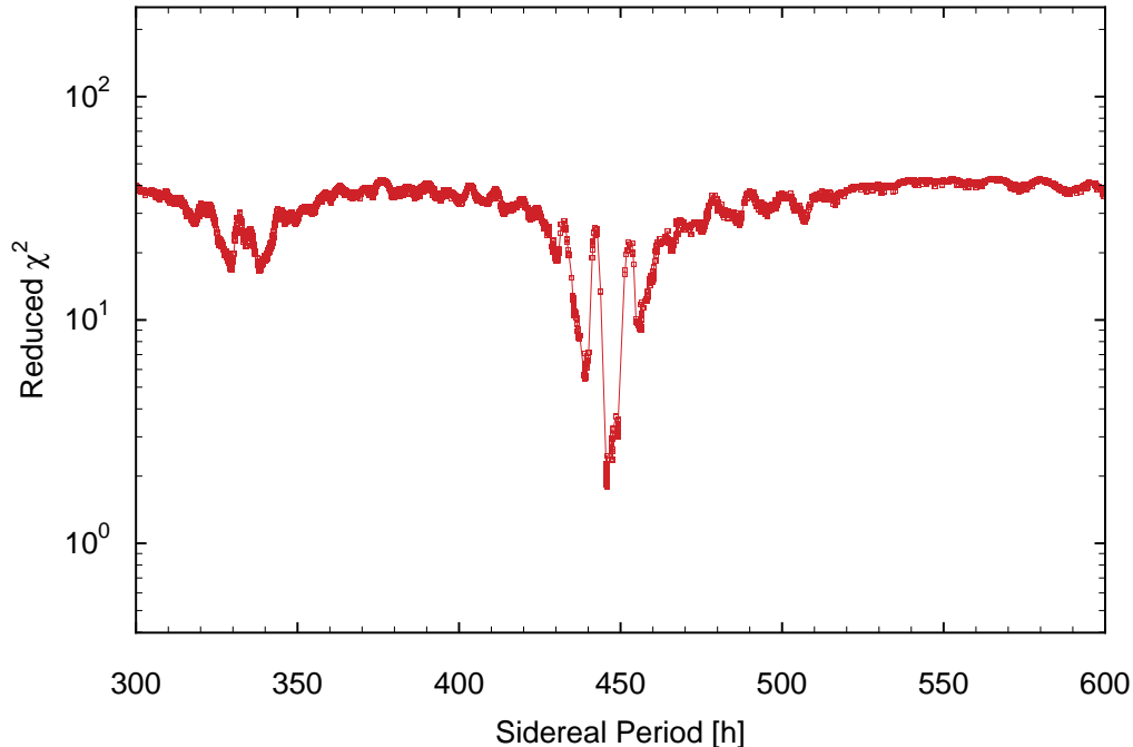
Figure 2. Result of the sidereal period scan. Each data point corresponds to a local-minimum solution obtained by using trial periods in the range between 300 h and 600 h as iteration start values for the sidereal period. The global minimum around 445.7 h corresponds to the best-fit solution.
