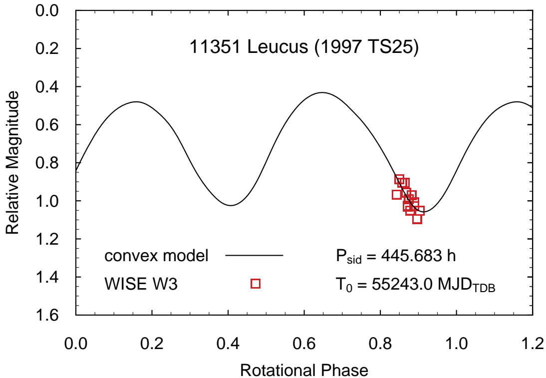
Figure 8. WISE observations (Grav et al. 2012) in the W3 12 \mu\text{m} thermal band are phased with a synthetic lightcurve from our convex model for the same epoch. Data points beyond rotational phase 1.0 are repeated for clarity. The magnitude scale for the WISE observations is arbitrarily offset to provide the best fit to the model curve. The plot shows that the WISE observations of Leucus were acquired near the lightcurve minimum.
