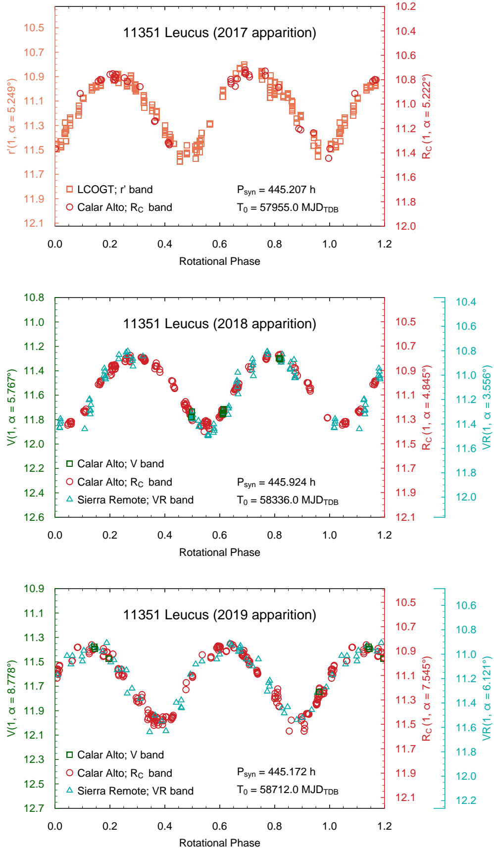
Figure 1. Composite lightcurves for the 2017, 2018 and 2019 apparitions. The data points are folded with the synodic periods listed in the respective graphs, with zero phase corresponding to the respective T_0 epochs. T_0 are one-leg, light-travel time corrected Modified Julian Dates (MJD) expressed in the TDB uniform time frame. The listed synodic periods are the exact numbers used for folding the composites, and as such, are reported without uncertainty. Data points beyond rotation phase 1.0 are repeated for clarity. The magnitudes are reduced to 1 au from the observer and from the Sun and to the respective reference phase angles by using a nominal linear phase coefficient \beta = 0.0395 \text{ mag}/^\circ .
