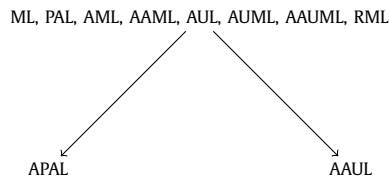
Fig. 4. The relative expressivity of the update logics discussed in the paper. Arrows indicate increasing expressivity. Absence of arrows indicates incomparable expressivity.
