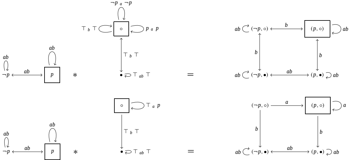
Fig. 2. Different ways of Anne learning that p .
