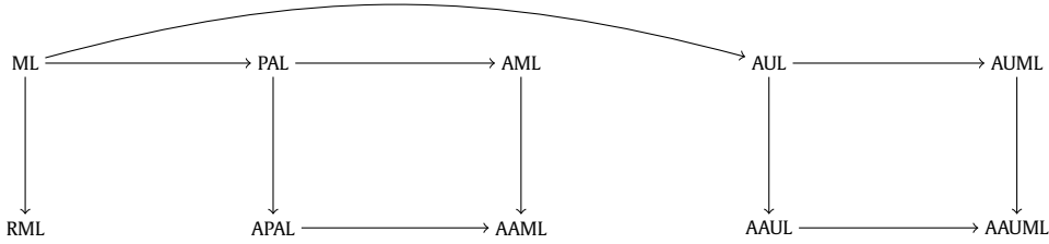
Fig. 1. An overview of update logics discussed in the paper. Horizontal arrows informally represent more complex updates. Vertical arrows informally represent quantification over updates. The arrows can be interpreted as syntactic extensions (modulo the names of quantifiers) or as semantic generalizations. Assume transitive closure.
