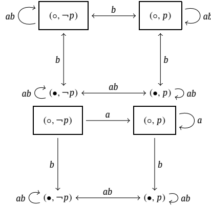
Fig. 8. From arrow updates to action models – example.
