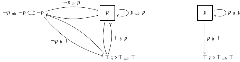
Fig. 7. From action models to arrow updates – example.
