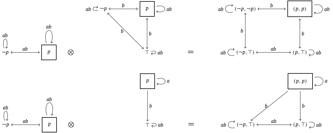
Fig. 6. Examples of action model execution.
