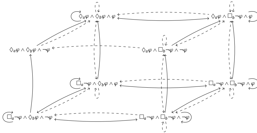
Fig. 9. Action model for lying.
