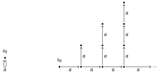
Fig. 10. Arbitrary arrow updates and refinements are incomparable.
